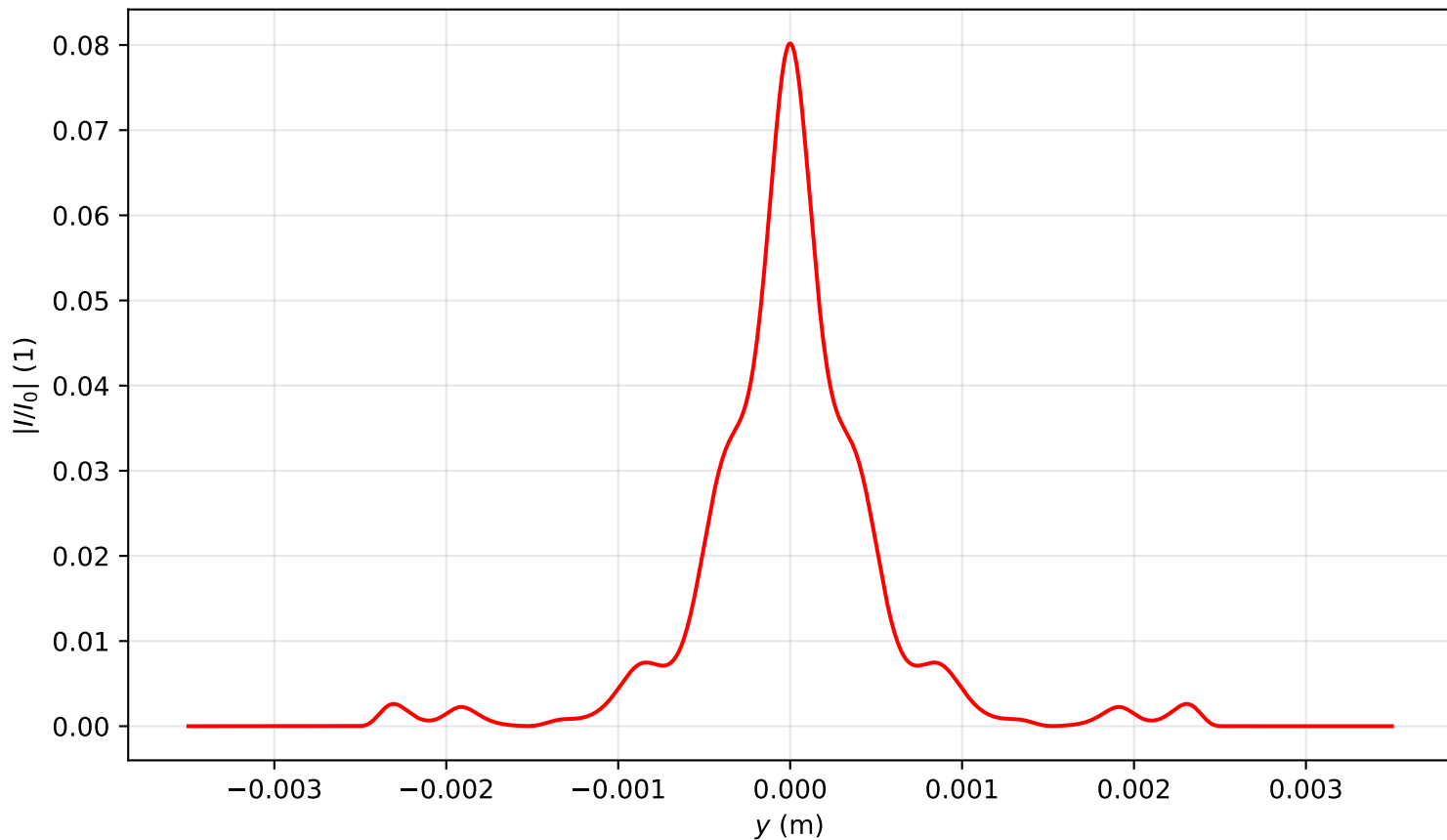
Intensity profile I(x=0, y, z=3.184)/I_0 , P_{in}=16.0P_{cr} , artificial time
