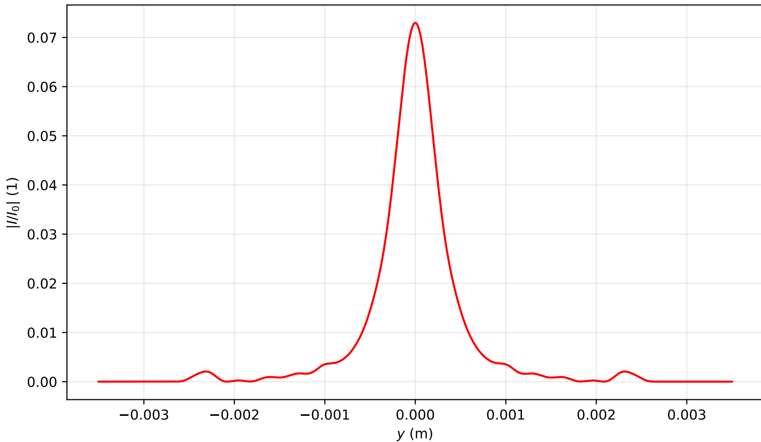
Intensity profile I(x=0, y, z=3.981)/I_0 , P_{in}=16.0P_{cr} , artificial time
