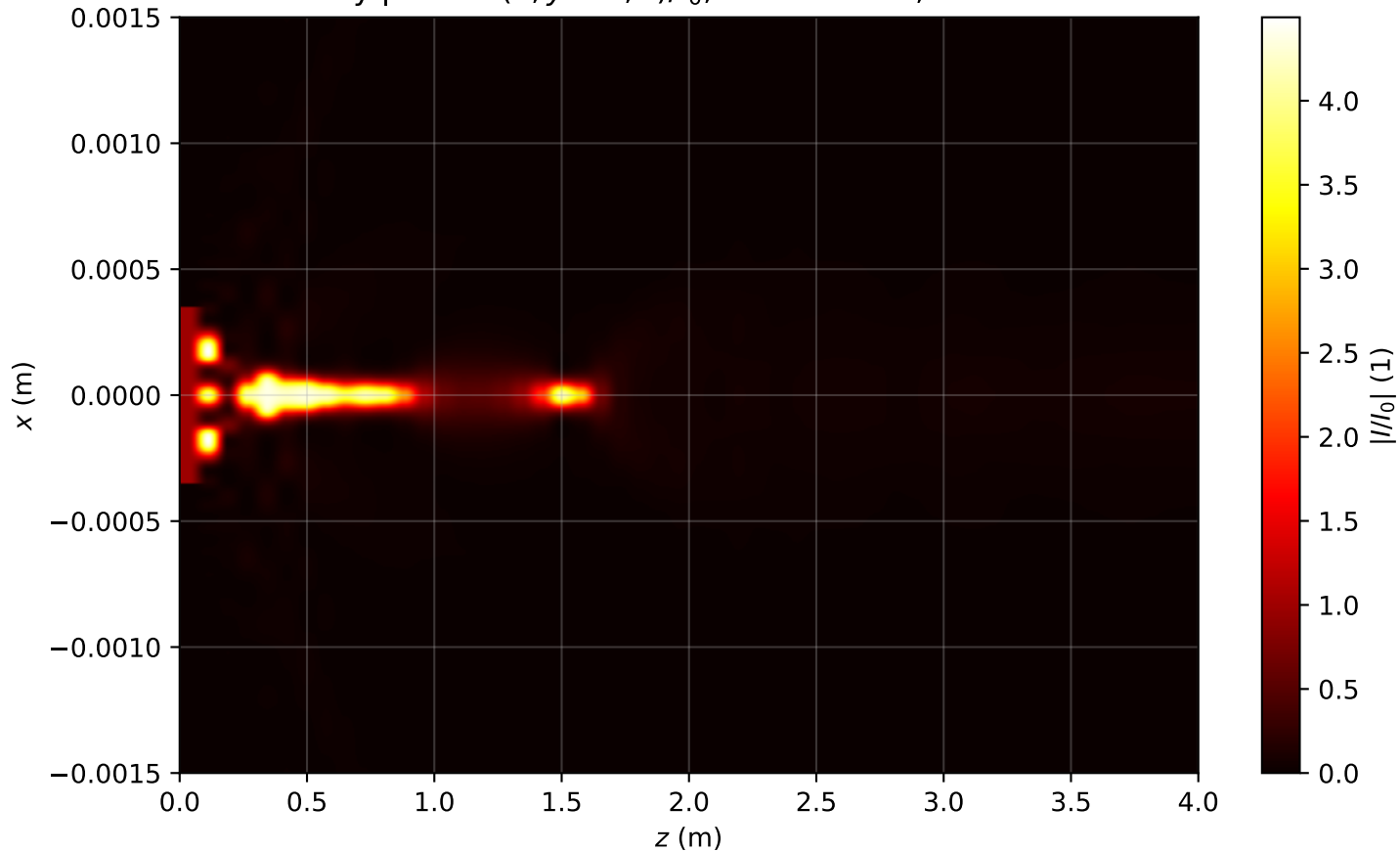
Intensity profile I(x, y = 0, z)/I_0 , P_{in}=16.0P_{cr} , artificial time
