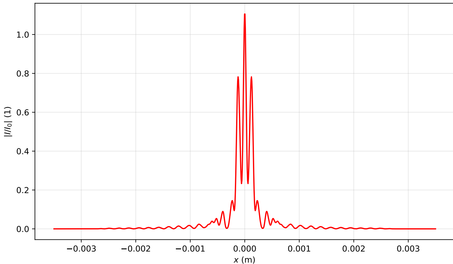
Intensity profile I(x, y = 0, z = 0.159)/I_0 , P_{in}=17.0P_{cr} , artificial time
