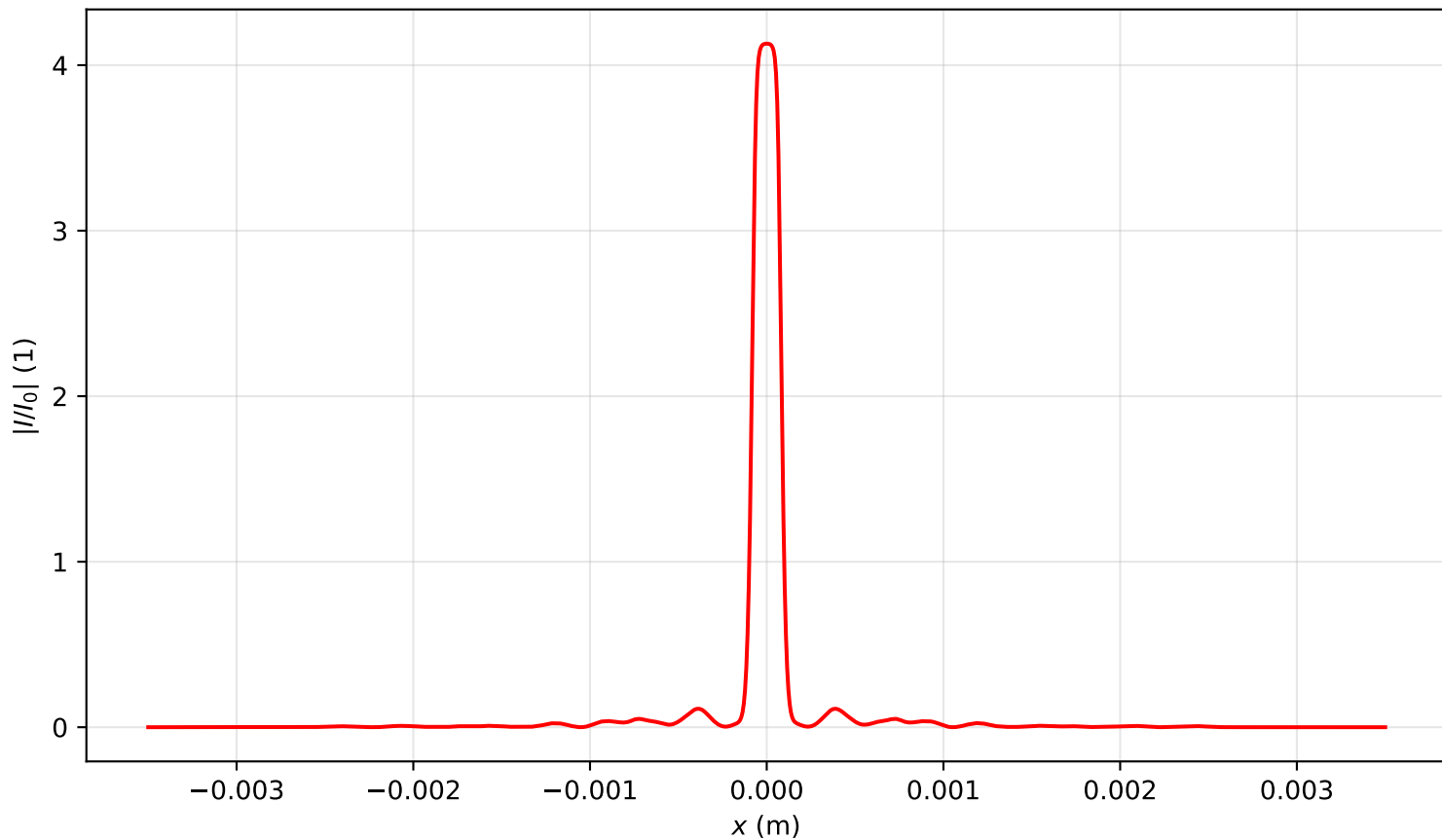
Intensity profile I(x, y = 0, z = 0.318)/I_0 , P_{in}=17.0P_{cr} , artificial time
