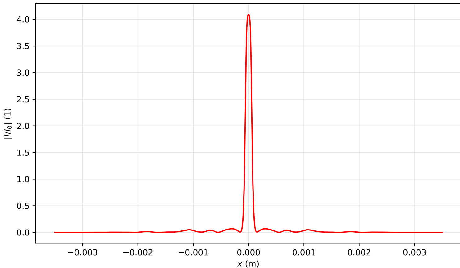
Intensity profile I(x, y = 0, z = 0.478)/I_0 , P_{in}=17.0P_{cr} , artificial time
