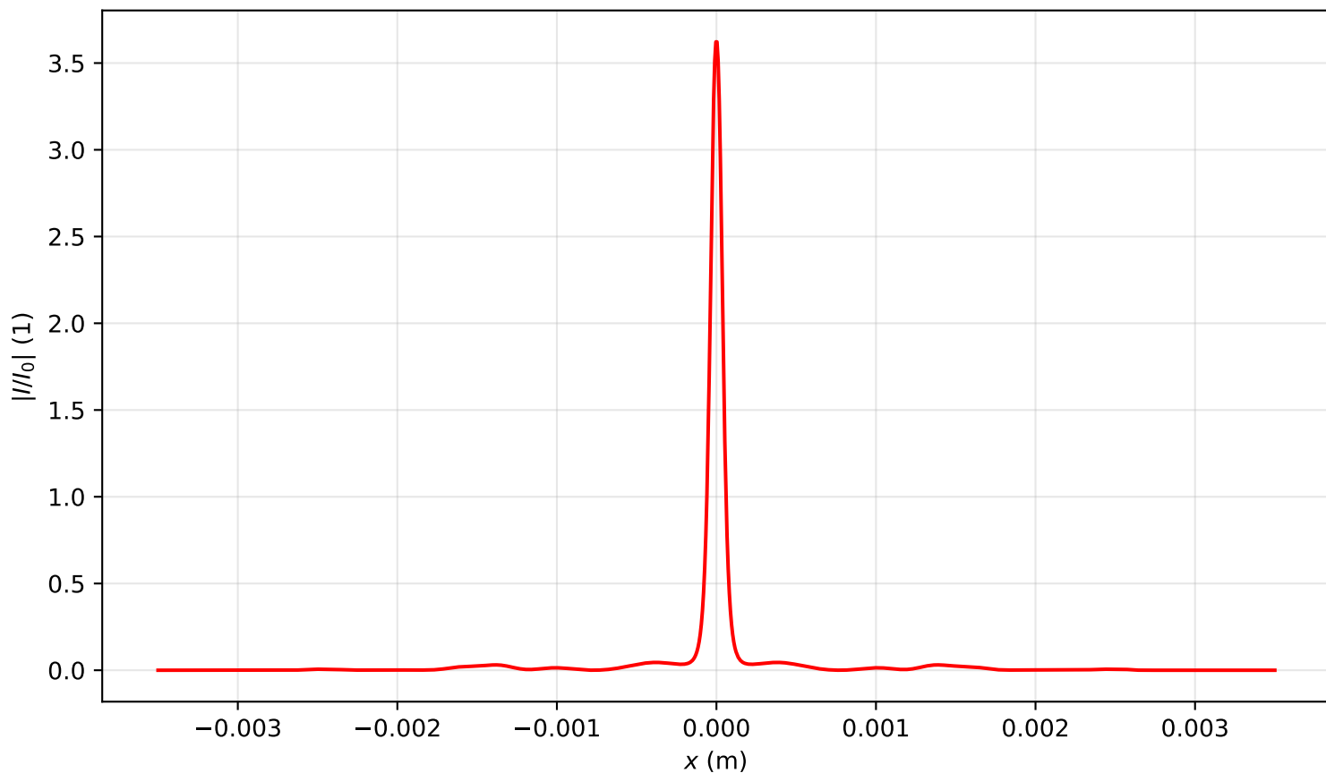
Intensity profile I(x, y = 0, z = 0.637)/I_0 , P_{in}=17.0P_{cr} , artificial time
