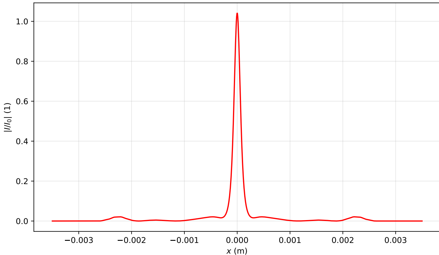
Intensity profile I(x, y = 0, z = 0.955)/I_0 , P_{in}=17.0P_{cr} , artificial time
