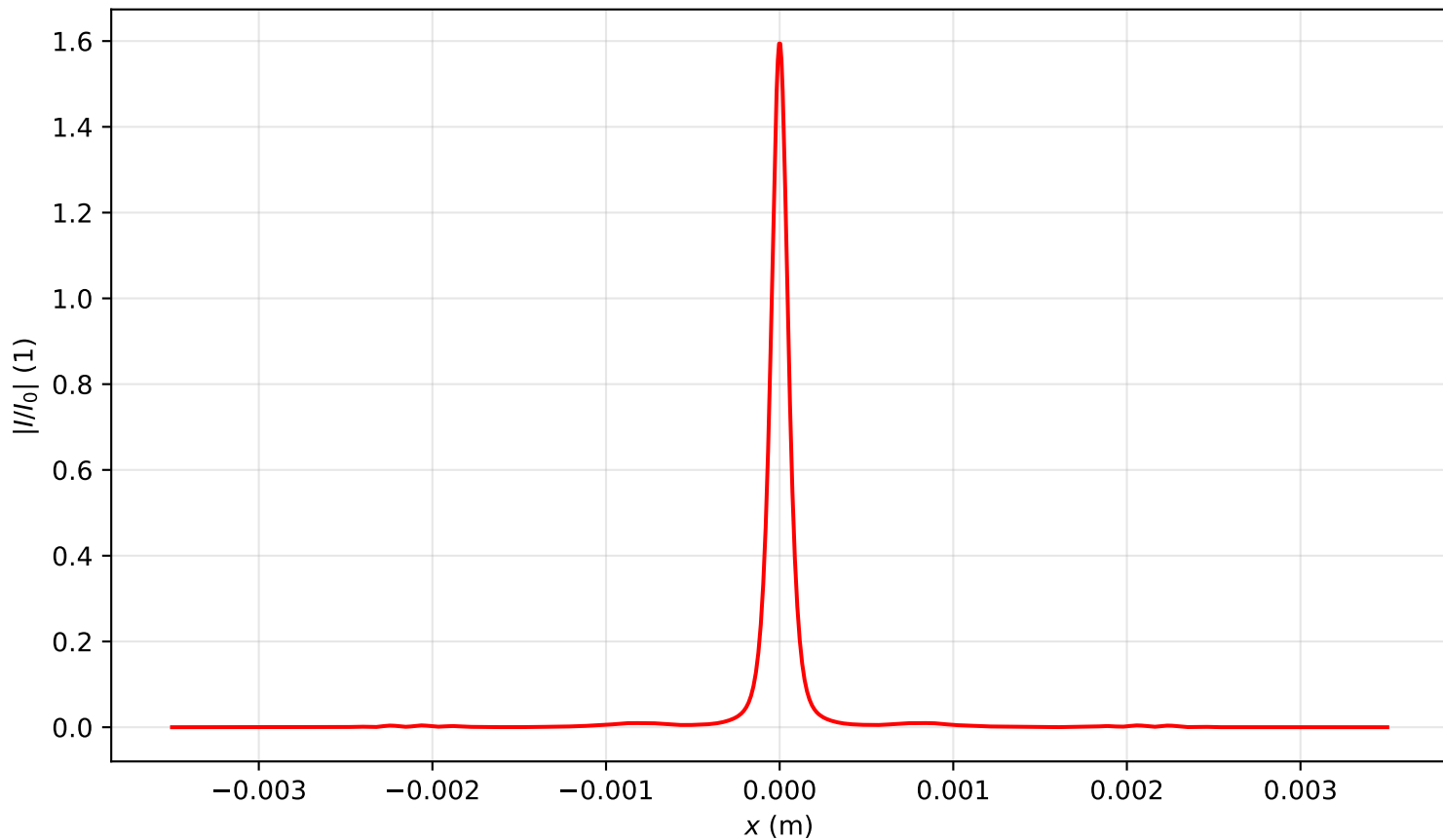
Intensity profile I(x, y = 0, z = 1.274)/I_0 , P_{in}=17.0P_{cr} , artificial time
