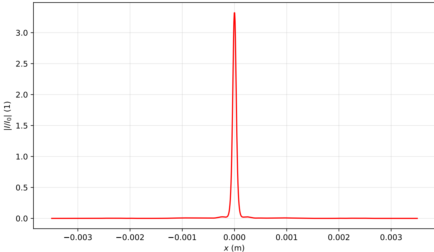
Intensity profile I(x, y = 0, z = 1.433)/I_0 , P_{in}=17.0P_{cr} , artificial time
