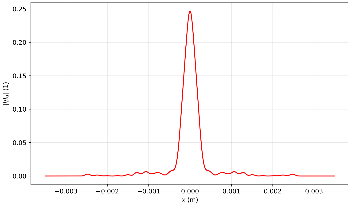
Intensity profile I(x, y = 0, z = 1.592)/I_0 , P_{in}=17.0P_{cr} , artificial time
