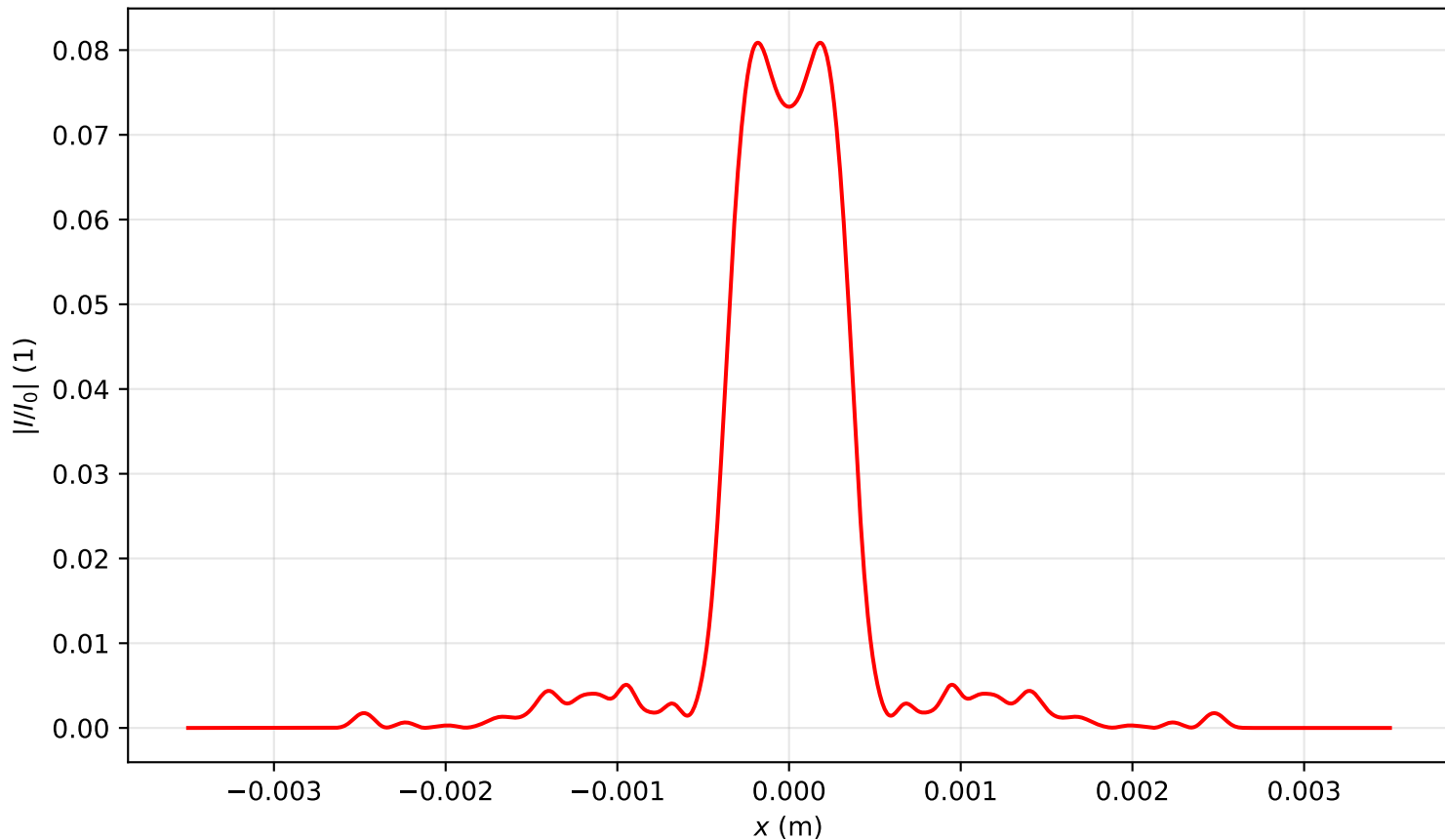
Intensity profile I(x, y = 0, z = 1.751)/I_0 , P_{in}=17.0P_{cr} , artificial time
