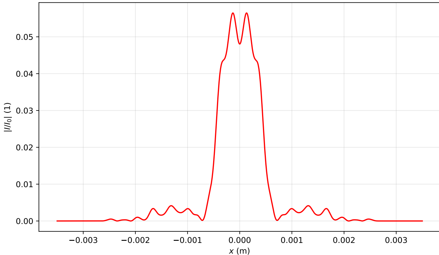
Intensity profile I(x, y = 0, z = 1.911)/I_0 , P_{in}=17.0\text{Pcr} , artificial time
