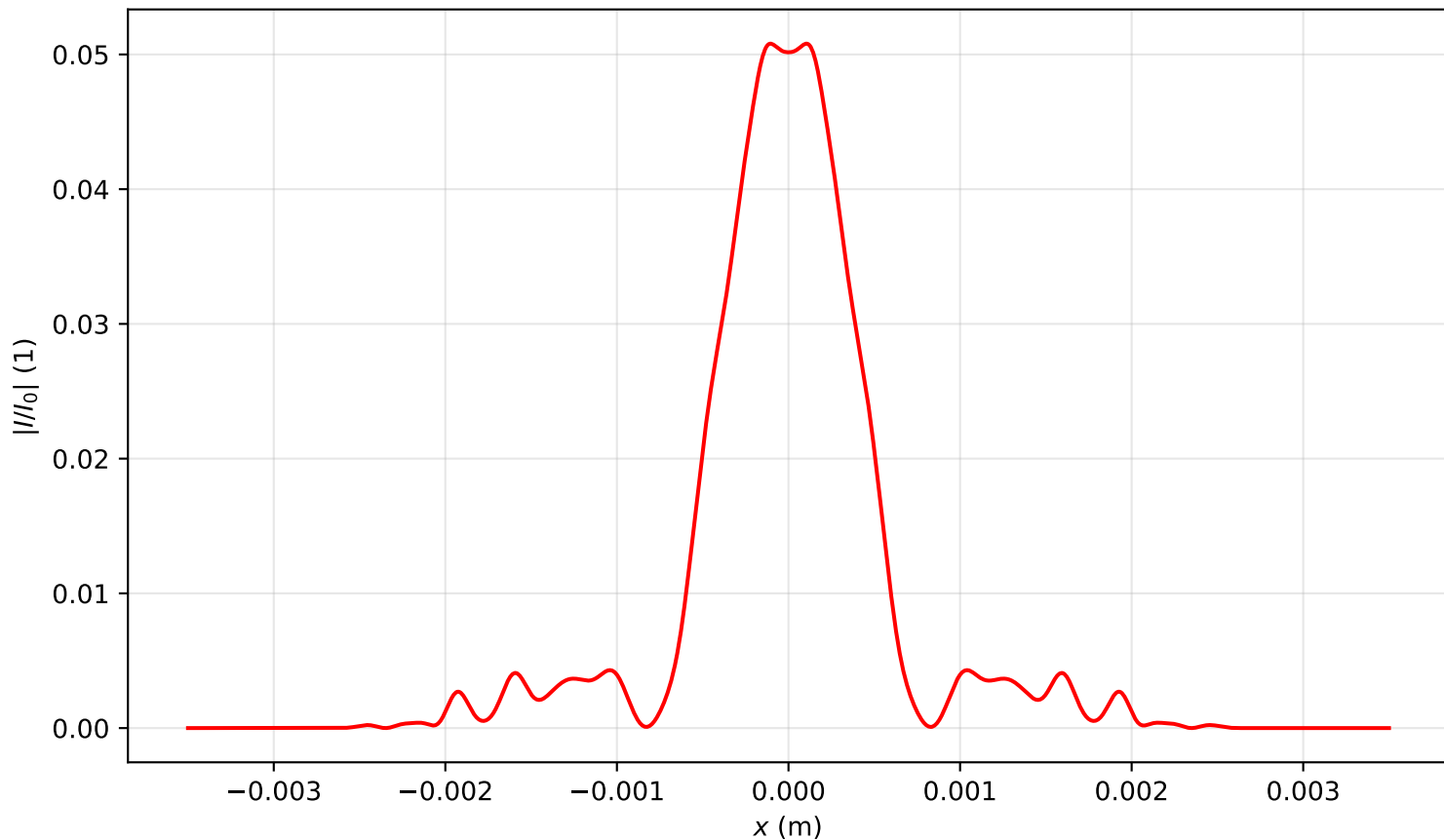
Intensity profile I(x, y = 0, z = 2.070)/I_0 , P_{in}=17.0P_{cr} , artificial time
