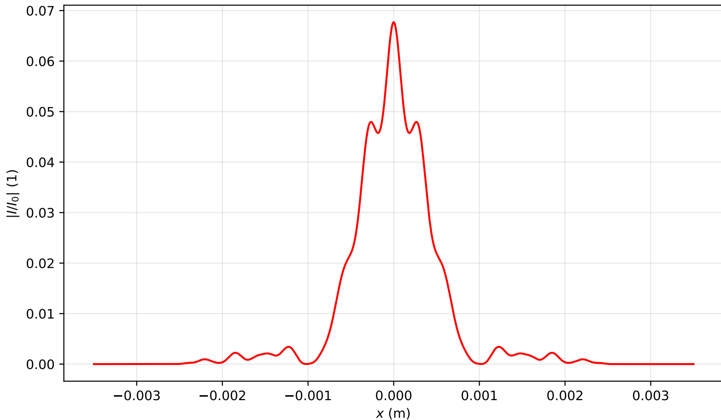
Intensity profile I(x, y = 0, z = 2.229)/I_0 , P_{in}=17.0P_{cr} , artificial time
