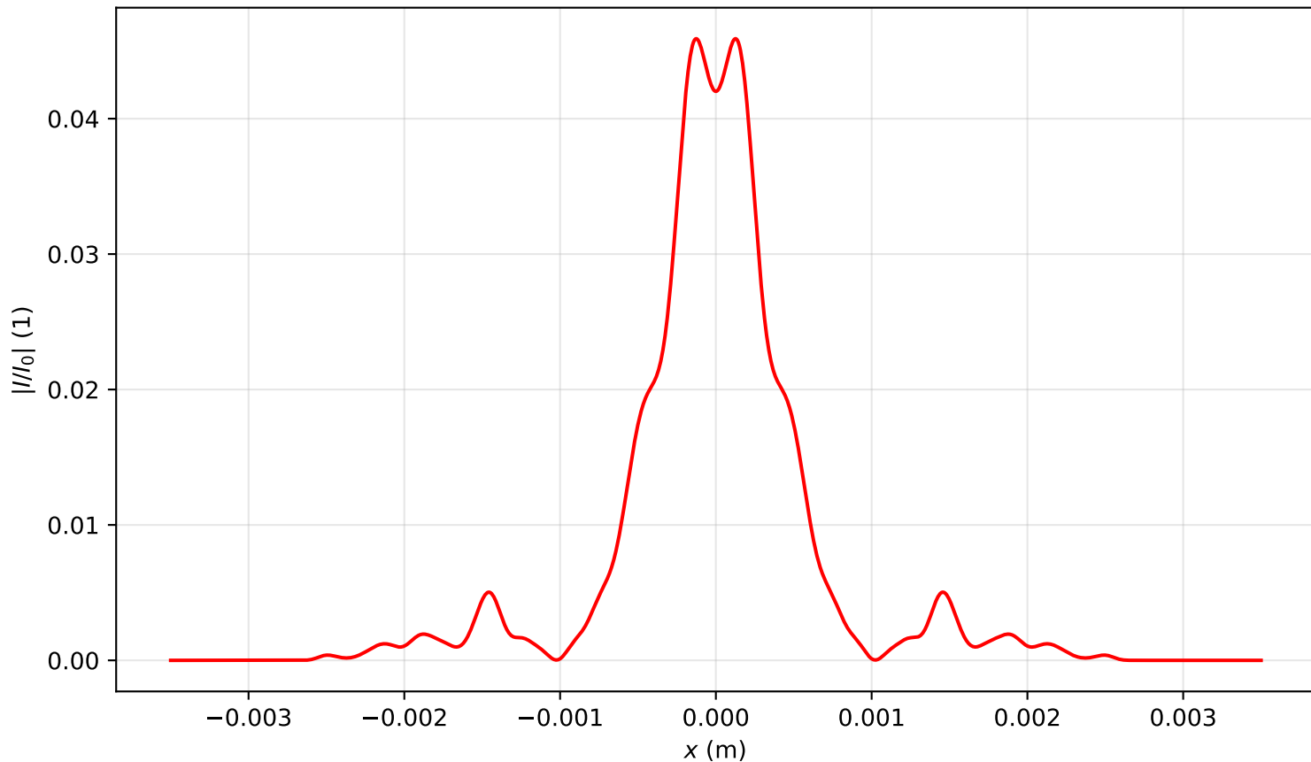
Intensity profile I(x, y = 0, z = 2.388)/I_0 , P_{in}=17.0\text{Pcr} , artificial time
