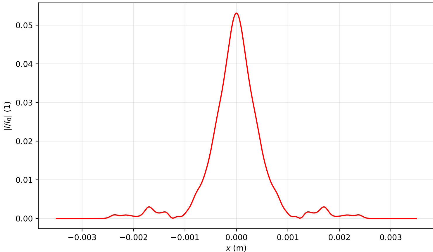
Intensity profile I(x, y = 0, z = 2.548)/I_0 , P_{in}=17.0\text{Pcr} , artificial time
