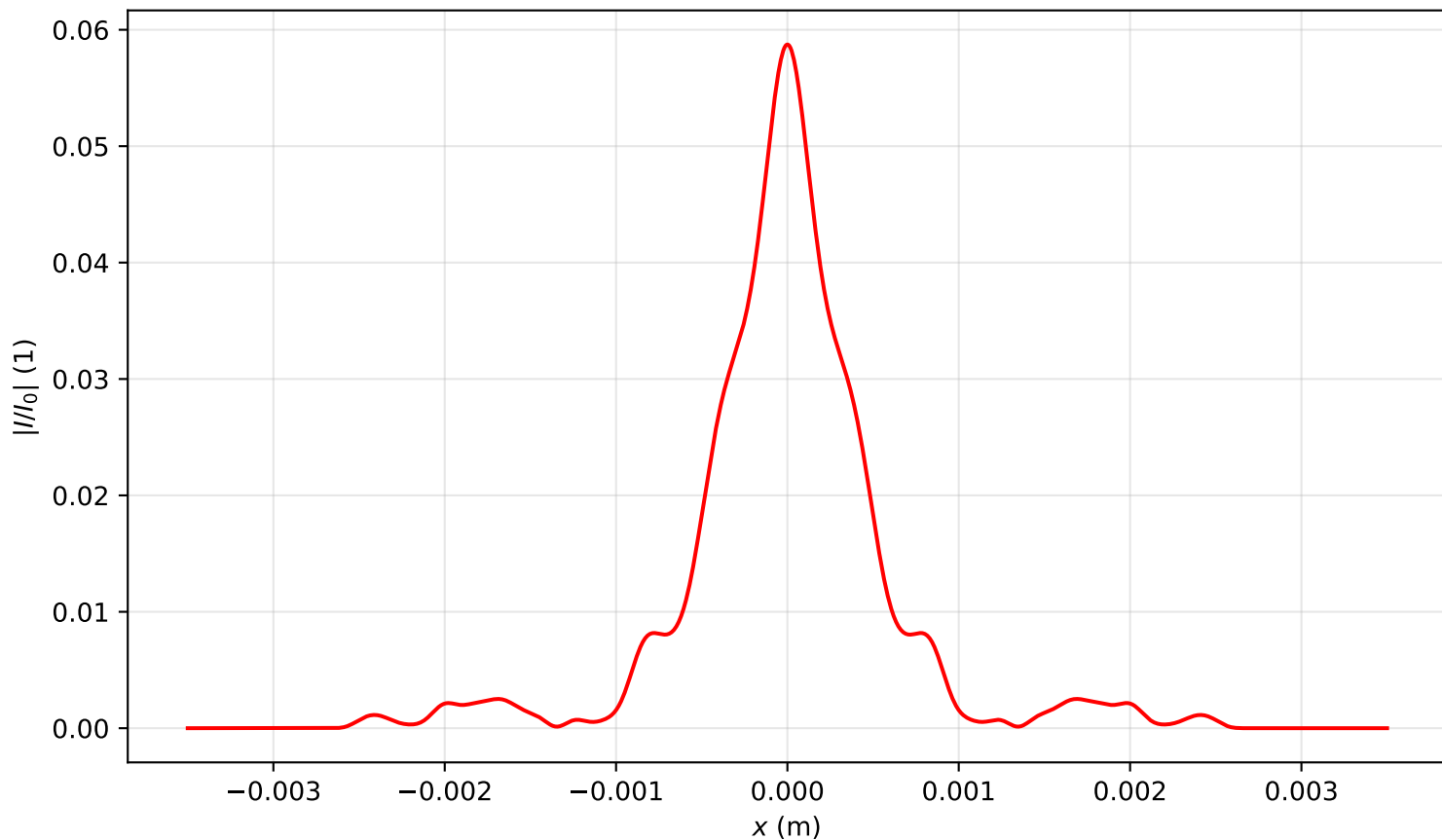
Intensity profile I(x, y = 0, z = 2.707)/I_0 , P_{in}=17.0\text{Pcr} , artificial time
