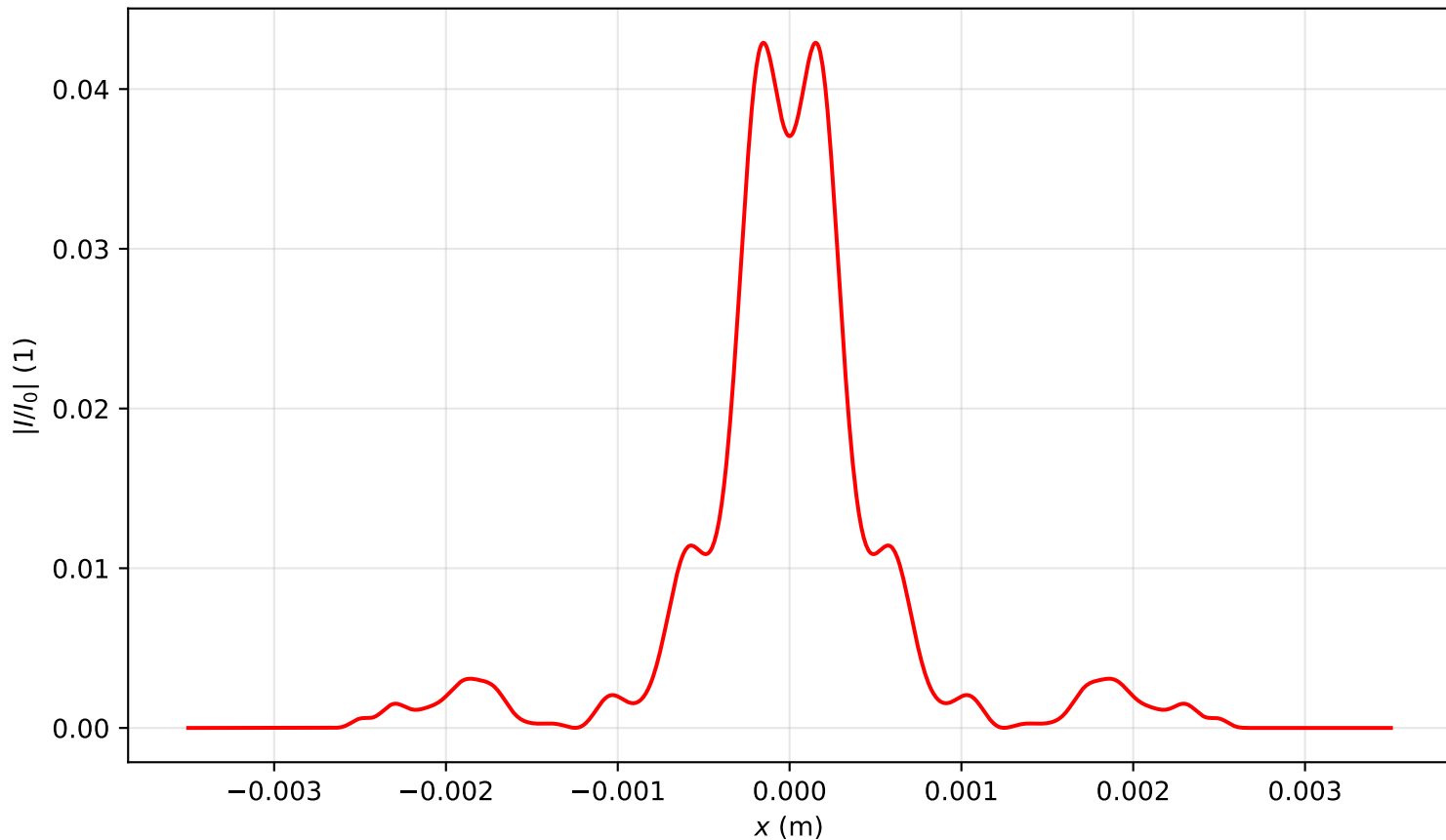
Intensity profile I(x, y = 0, z = 2.866)/I_0 , P_{in}=17.0\text{Pcr} , artificial time
