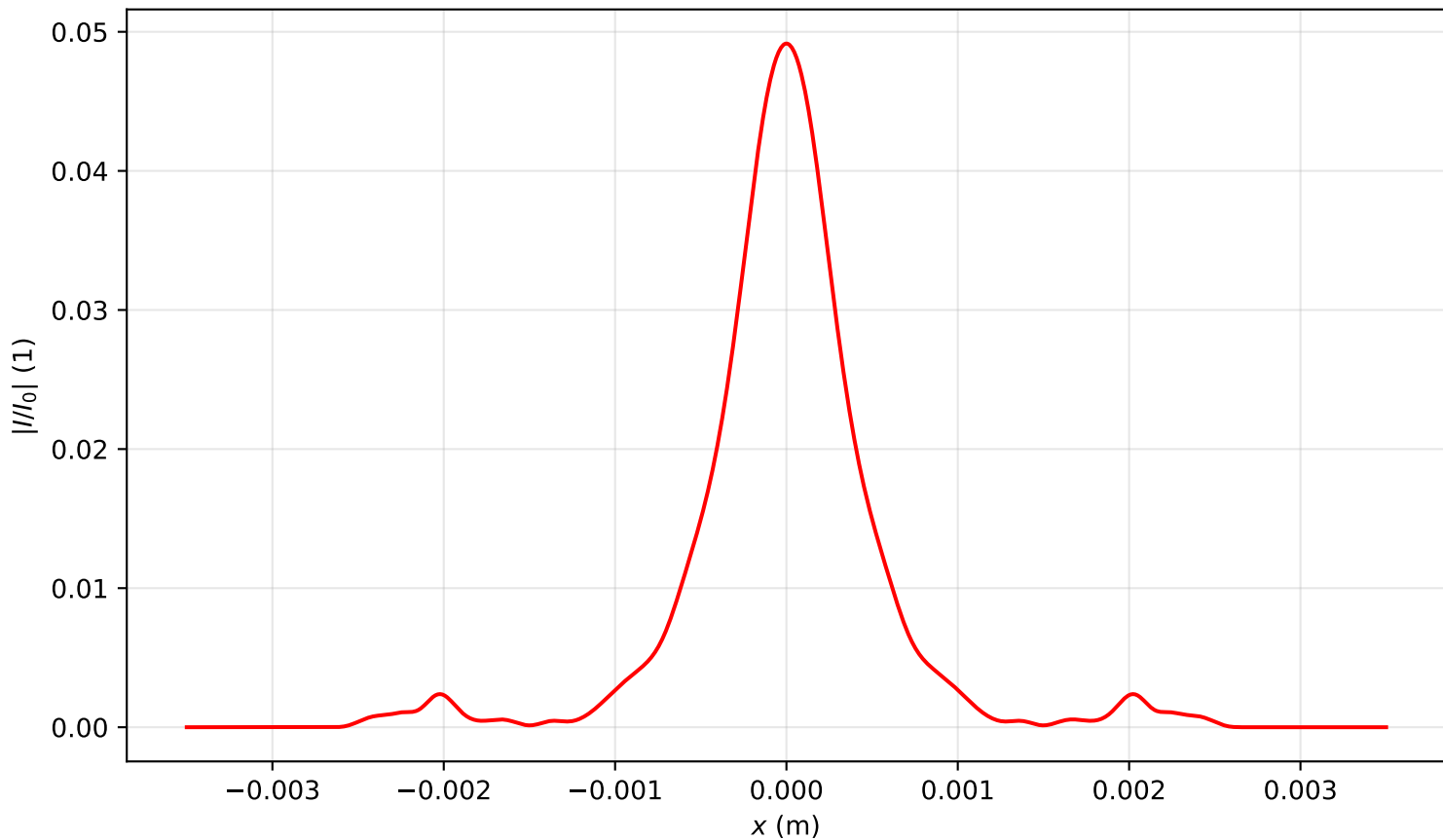
Intensity profile I(x, y = 0, z = 3.025)/I_0 , P_{in}=17.0P_{cr} , artificial time
