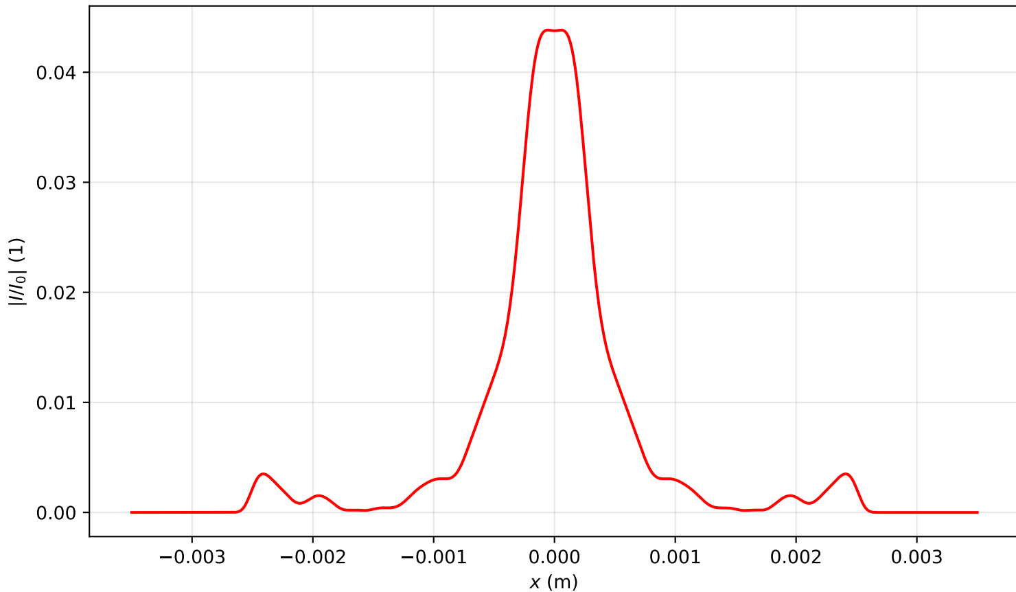
Intensity profile I(x, y = 0, z = 3.344)/I_0 , P_{in}=17.0P_{cr} , artificial time
