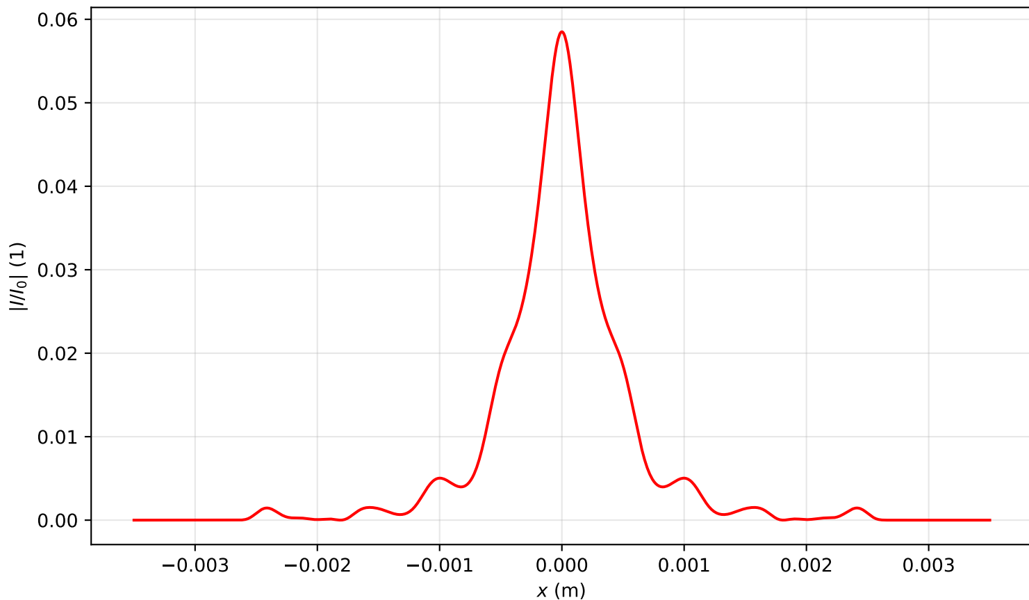
Intensity profile I(x, y = 0, z = 3.821)/I_0 , P_{in}=17.0P_{cr} , artificial time
