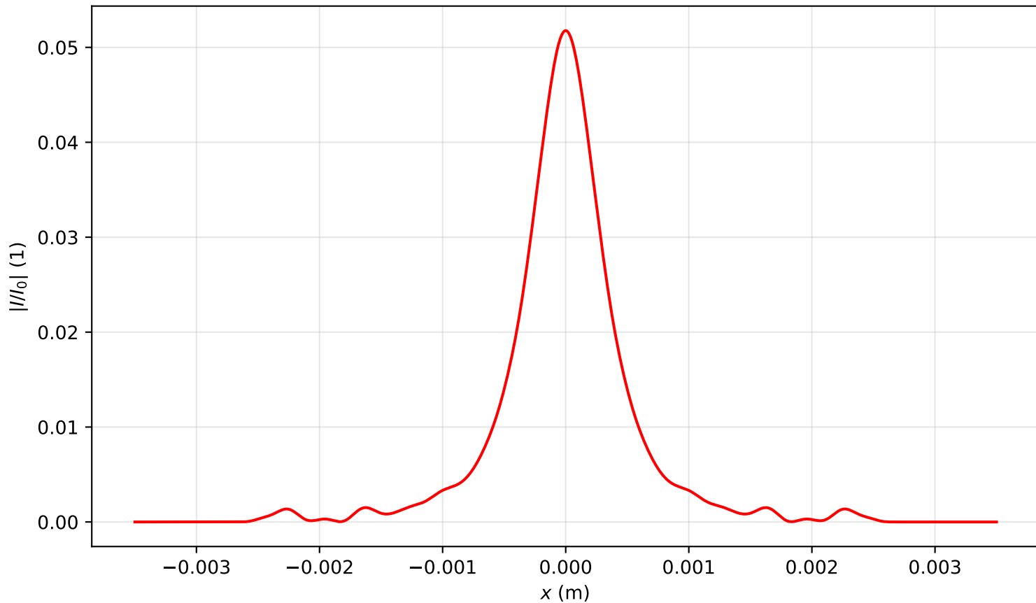
Intensity profile I(x, y = 0, z = 3.981)/I_0 , P_{in}=17.0\text{Pcr} , artificial time
