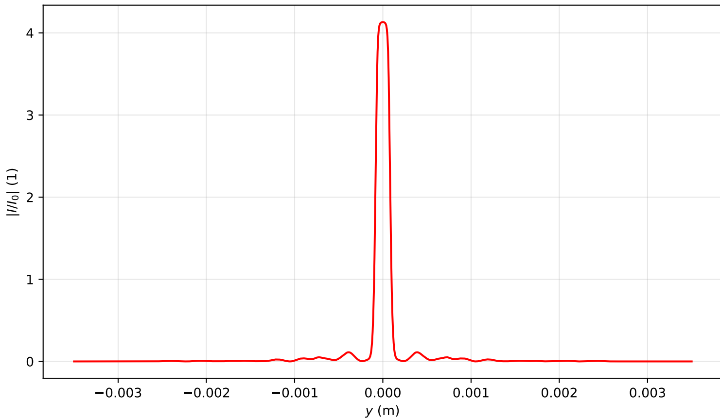
Intensity profile I(x=0, y, z=0.318)/I_0 , P_{in}=17.0P_{cr} , artificial time
