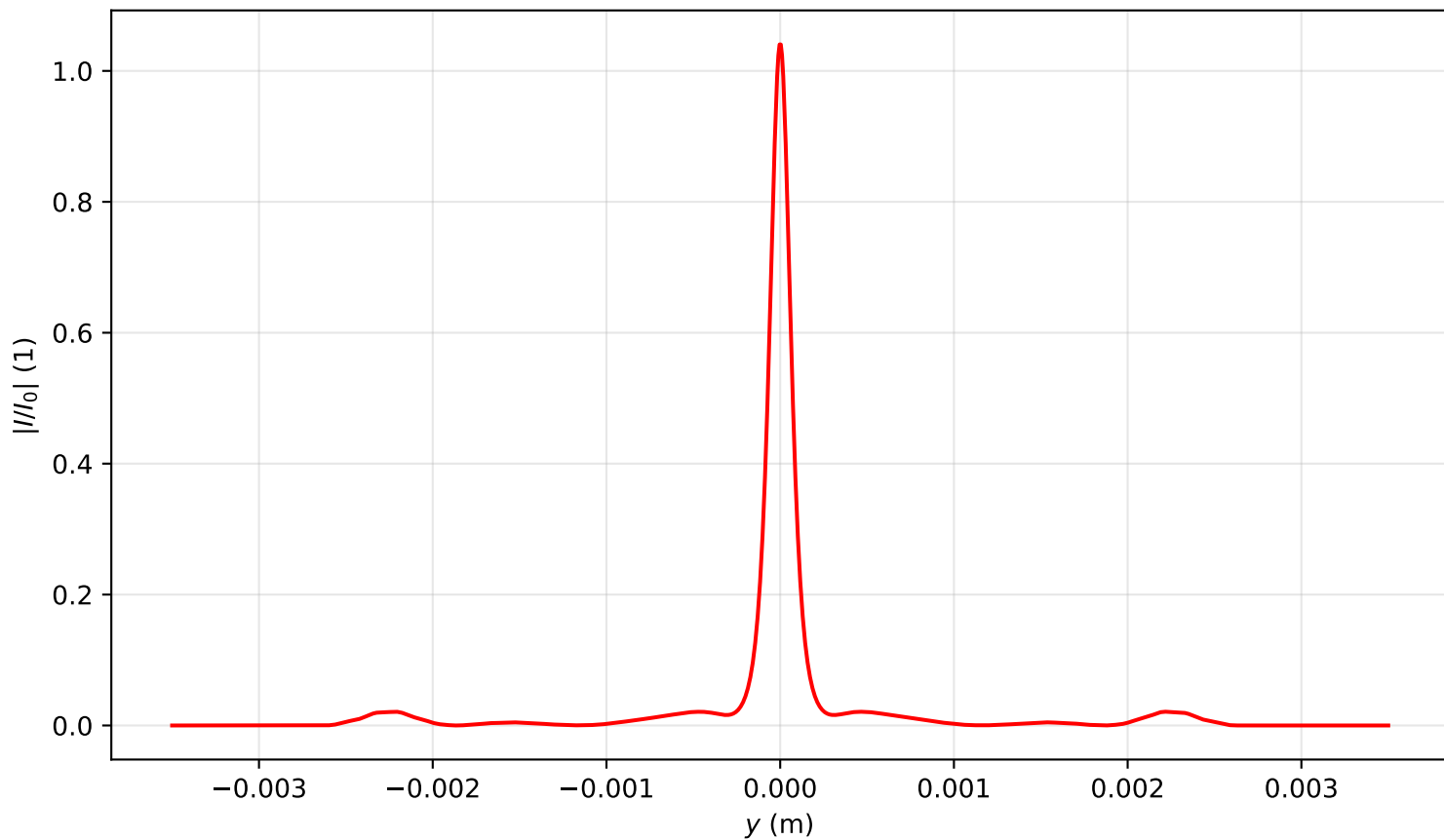
Intensity profile I(x=0, y, z=0.955)/I_0 , P_{in}=17.0P_{cr} , artificial time
