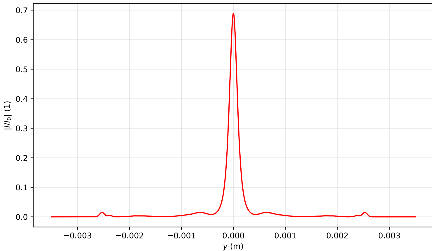
Intensity profile I(x=0, y, z=1.115)/I_0 , P_{in}=17.0P_{cr} , artificial time
