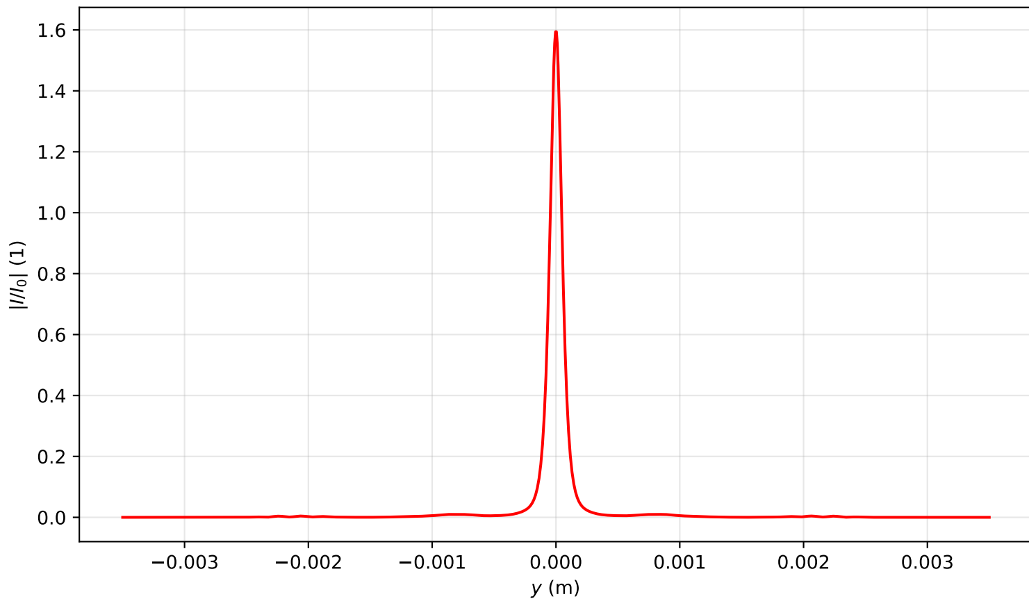
Intensity profile I(x=0, y, z=1.274)/I_0 , P_{in}=17.0\text{Pcr} , artificial time
