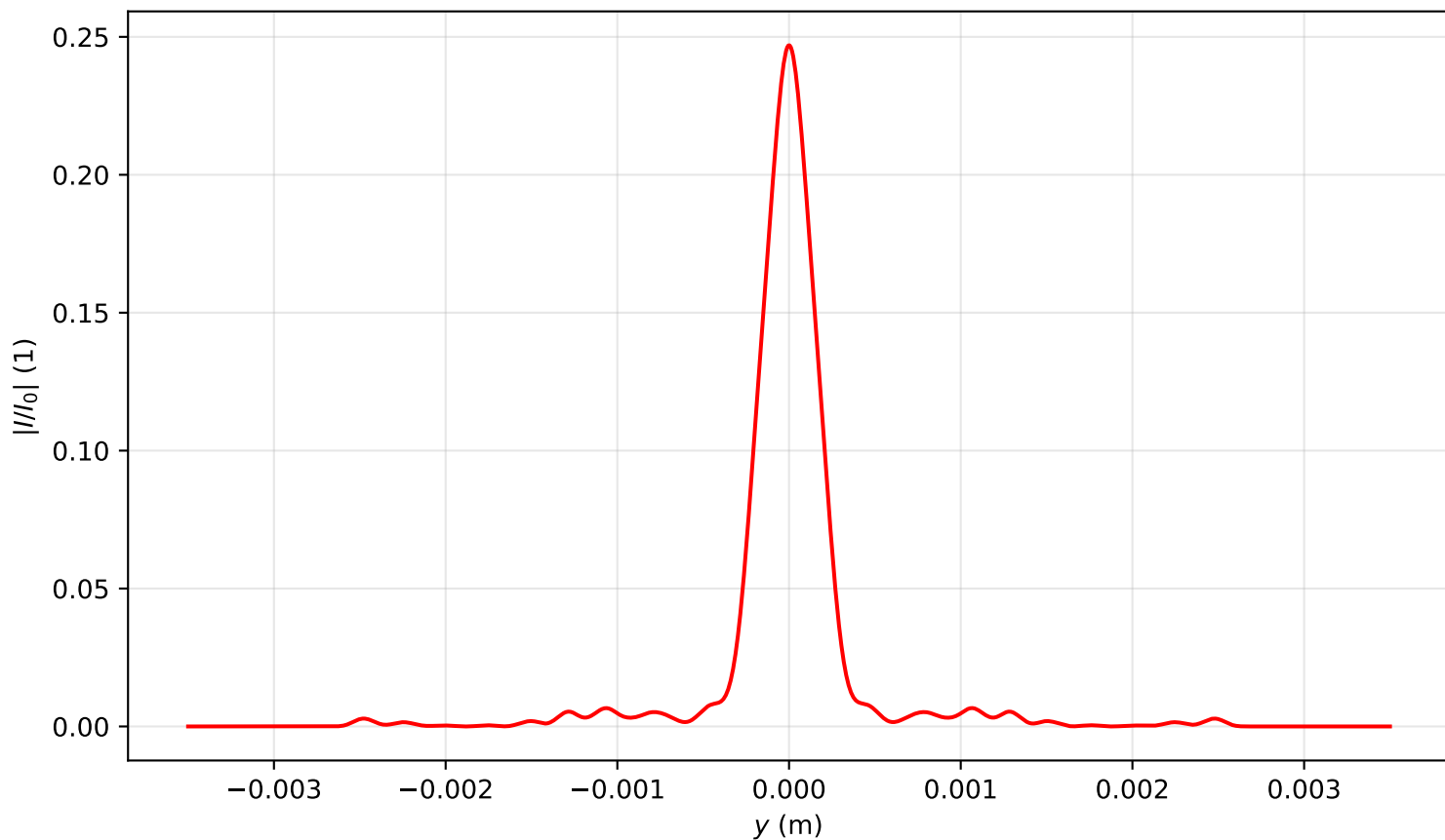
Intensity profile I(x=0, y, z=1.592)/I_0 , P_{in}=17.0P_{cr} , artificial time
