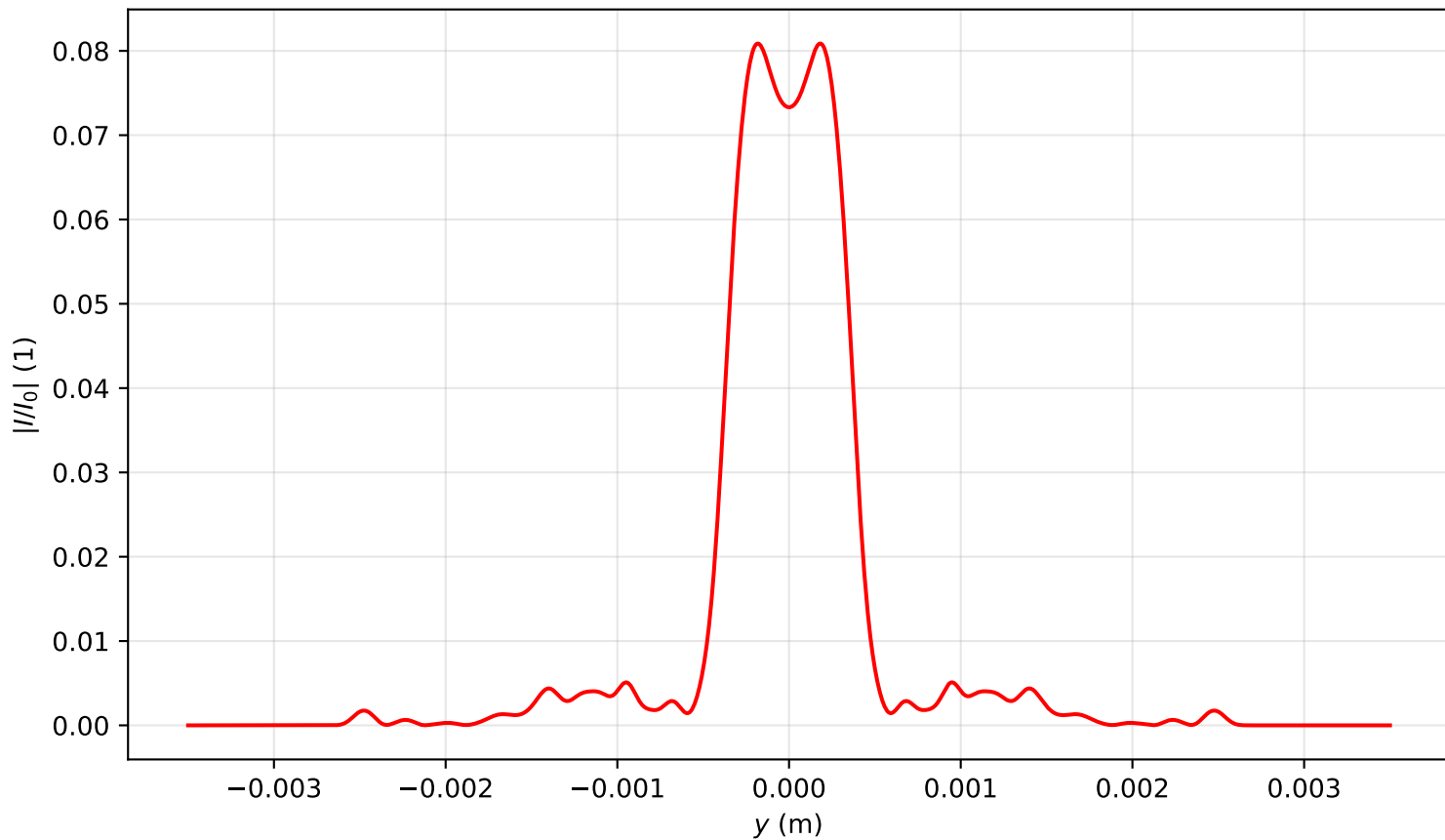
Intensity profile I(x = 0, y, z = 1.751)/I_0 , P_{in}=17.0\text{Pcr} , artificial time
