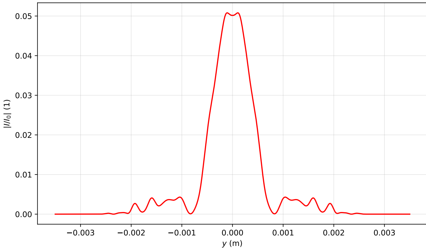
Intensity profile I(x = 0, y, z = 2.070)/I_0 , P_{in}=17.0P_{cr} , artificial time
