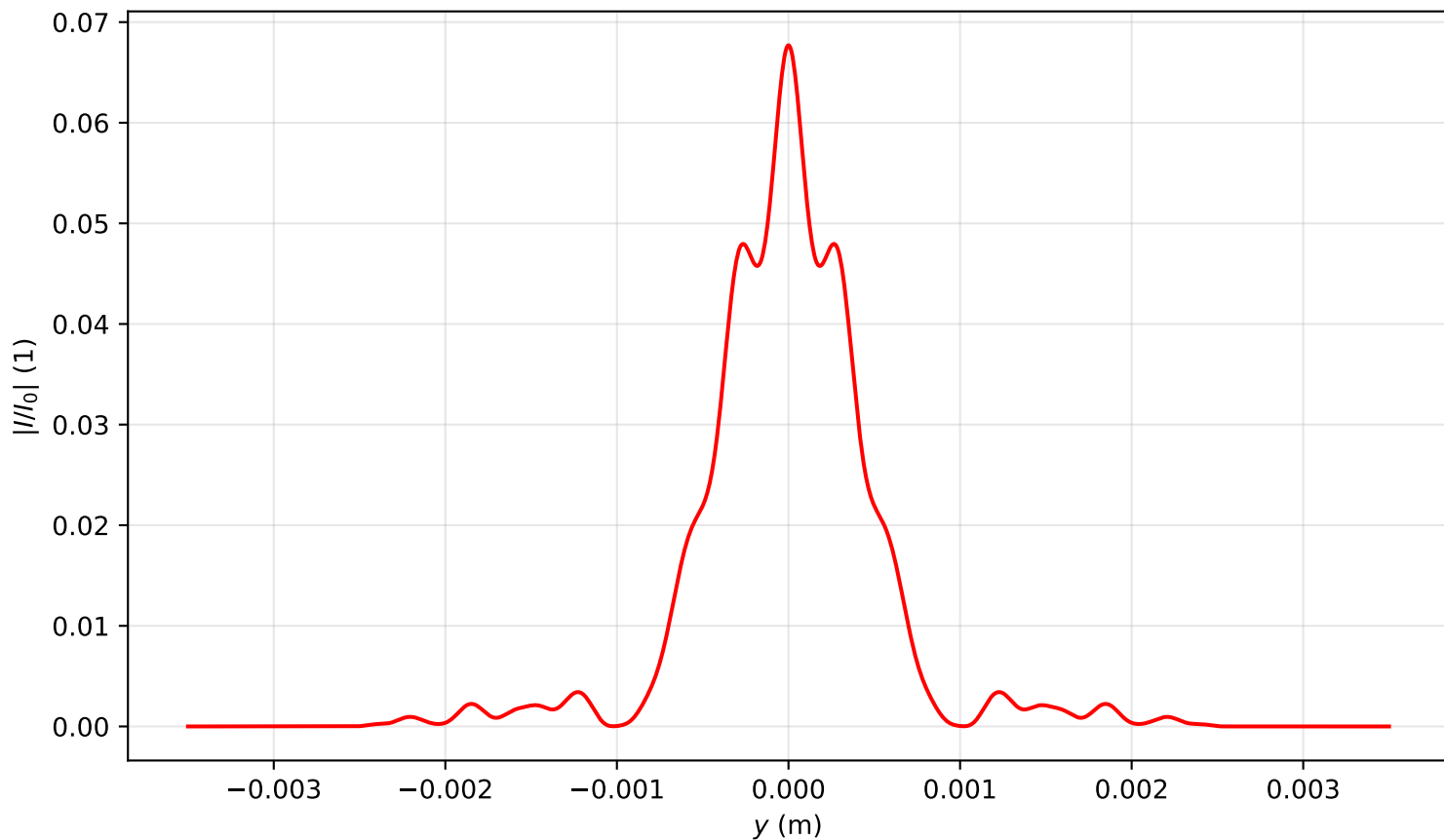
Intensity profile I(x = 0, y, z = 2.229)/I_0 , P_{in}=17.0P_{cr} , artificial time
