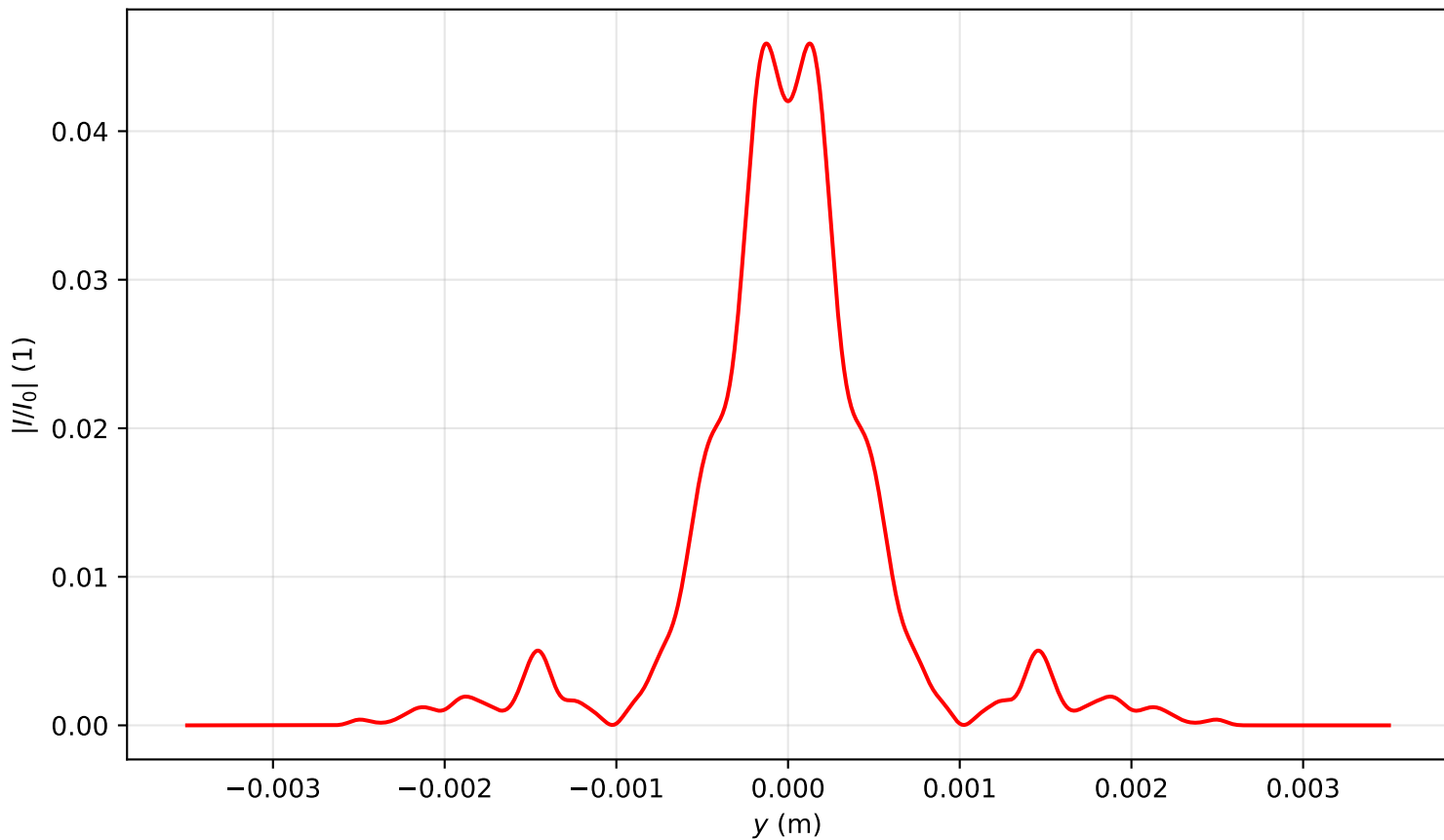
Intensity profile I(x=0, y, z=2.388)/I_0 , P_{in}=17.0\text{Pcr} , artificial time
