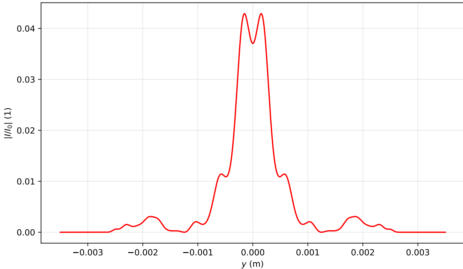
Intensity profile I(x = 0, y, z = 2.866)/I_0 , P_{in}=17.0\text{Pcr} , artificial time
