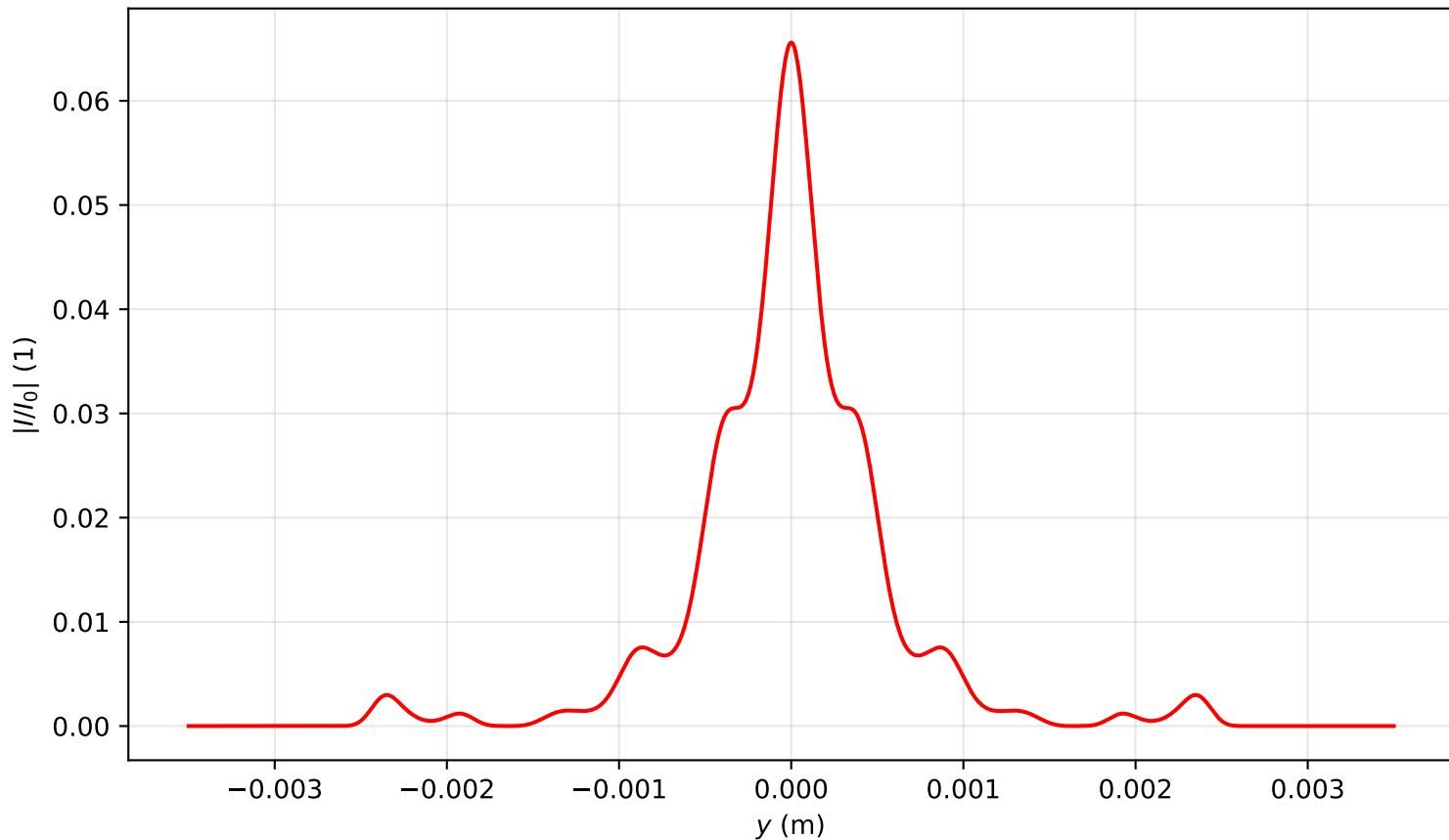
Intensity profile I(x = 0, y, z = 3.184)/I_0 , P_{in}=17.0P_{cr} , artificial time
