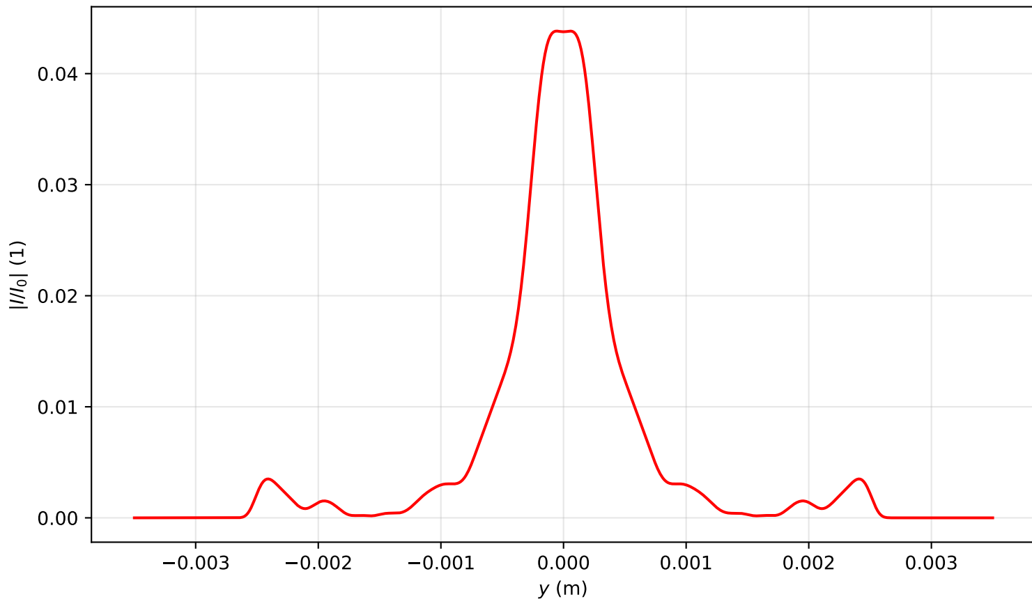
Intensity profile I(x = 0, y, z = 3.344)/I_0 , P_{in}=17.0P_{cr} , artificial time
