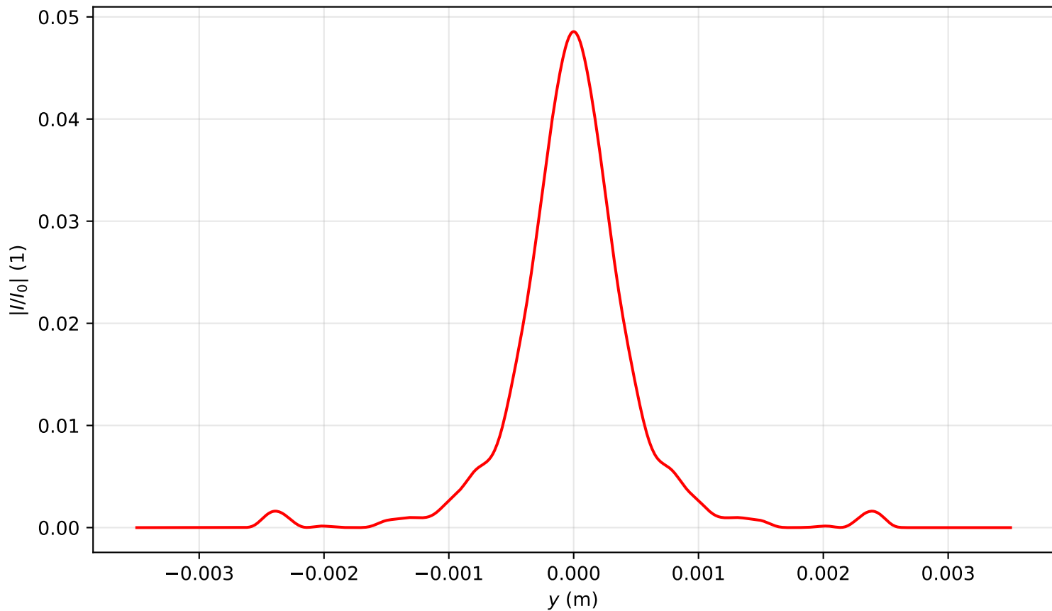
Intensity profile I(x = 0, y, z = 3.662)/I_0 , P_{in}=17.0P_{cr} , artificial time
