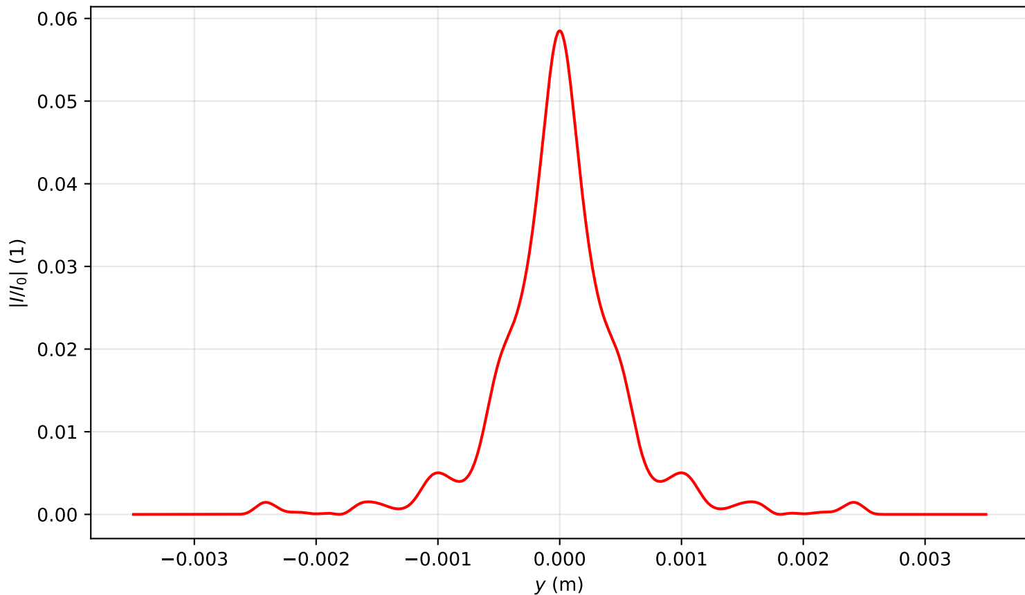
Intensity profile I(x = 0, y, z = 3.821)/I_0 , P_{in}=17.0P_{cr} , artificial time
