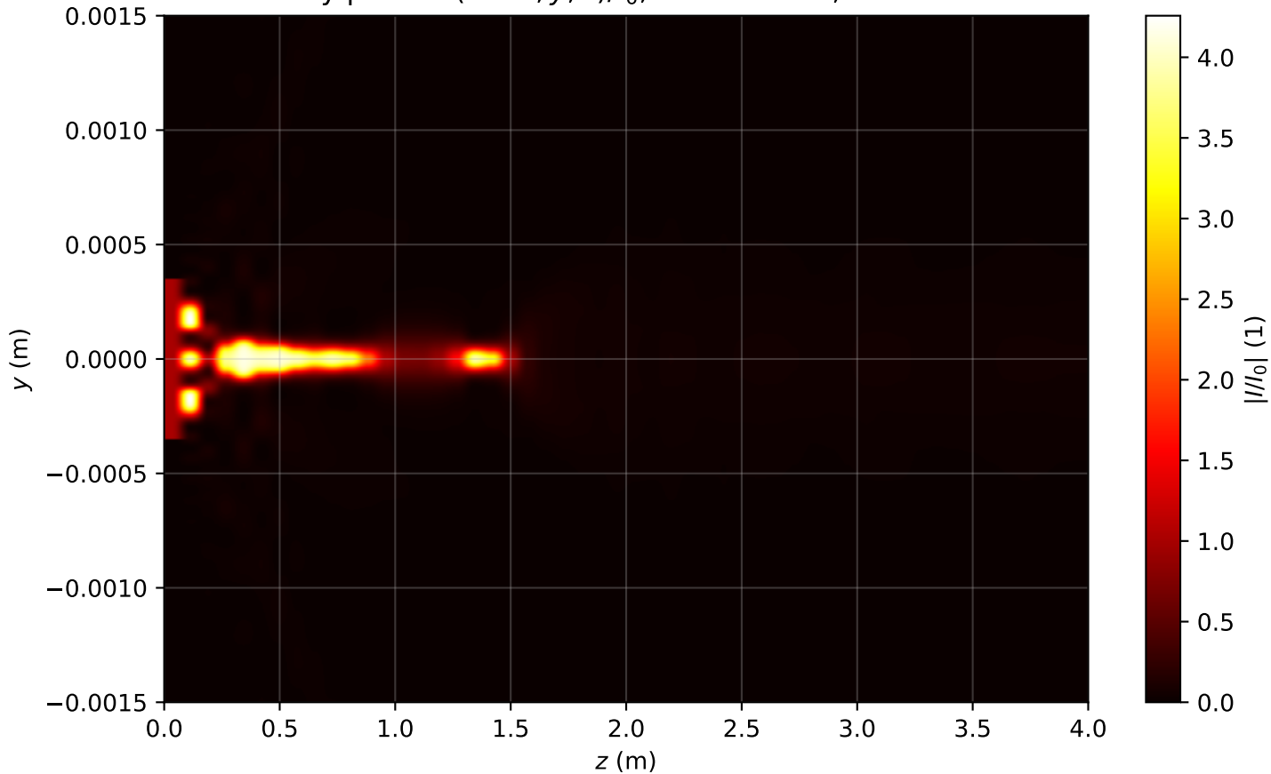
Intensity profile I(x=0, y, z)/I_0 , P_{in}=17.0\text{Pcr} , artificial time
