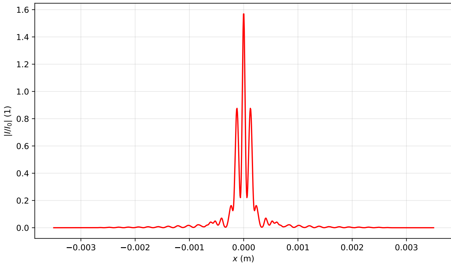
Intensity profile I(x, y = 0, z = 0.159)/I_0 , P_{in}=18.0P_{cr} , artificial time
