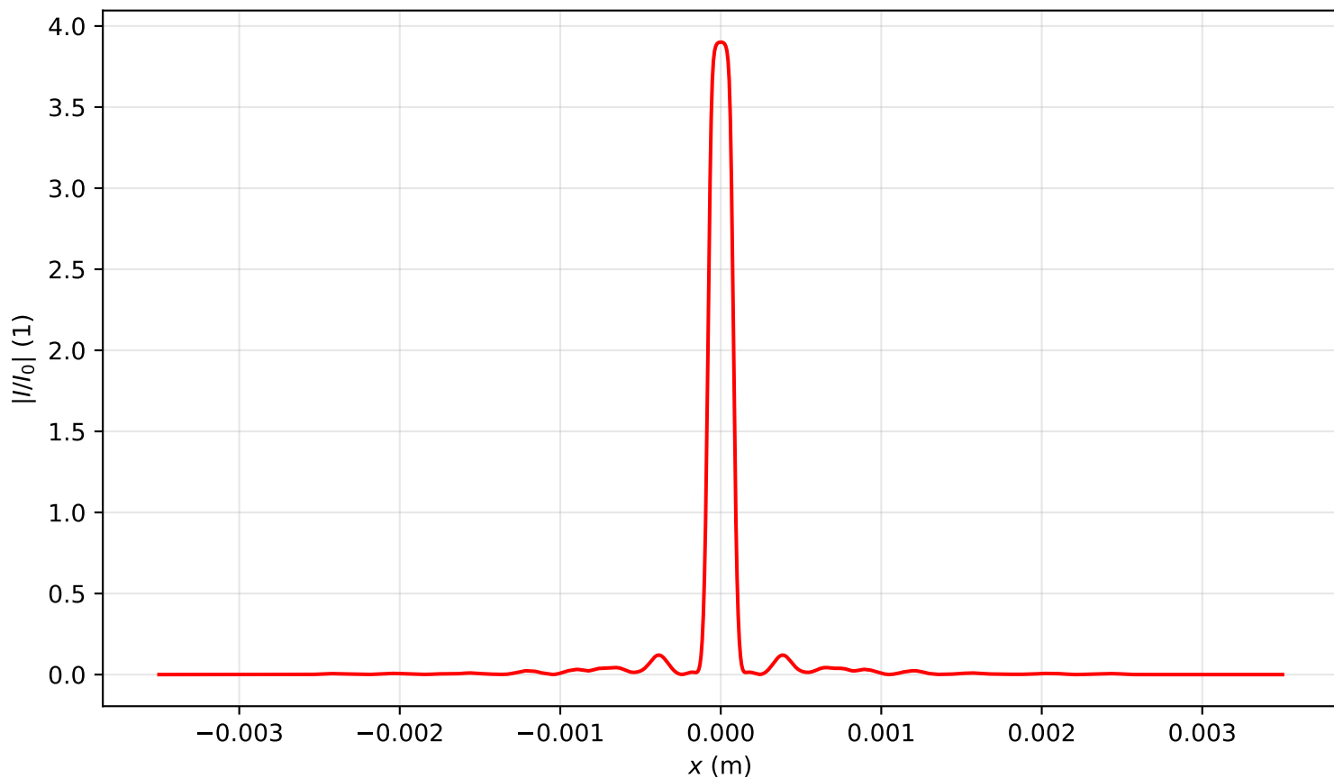
Intensity profile I(x, y = 0, z = 0.318)/I_0 , P_{in}=18.0P_{cr} , artificial time
