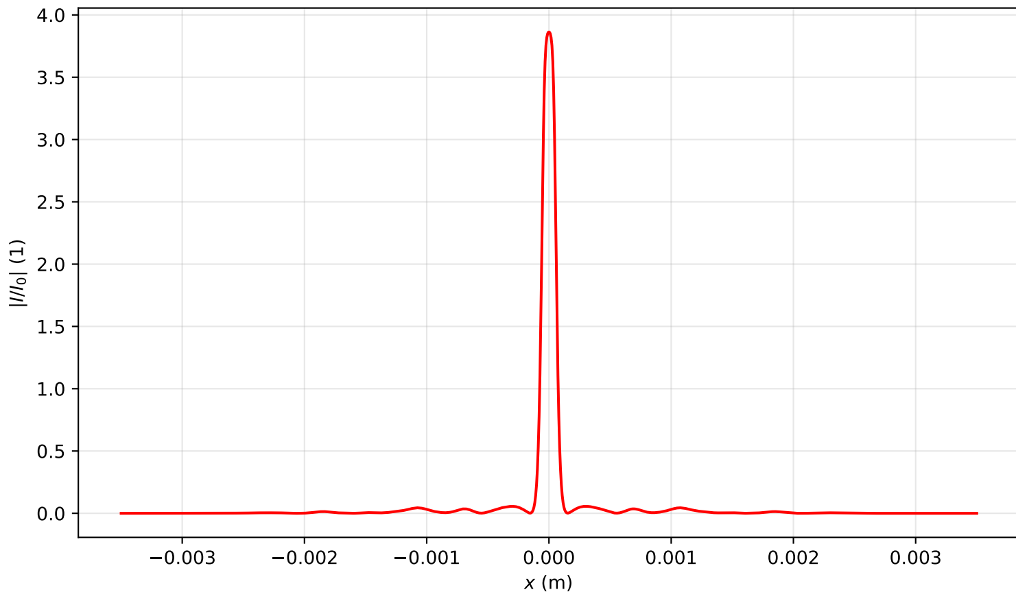
Intensity profile I(x, y = 0, z = 0.478)/I_0 , P_{in}=18.0P_{cr} , artificial time
