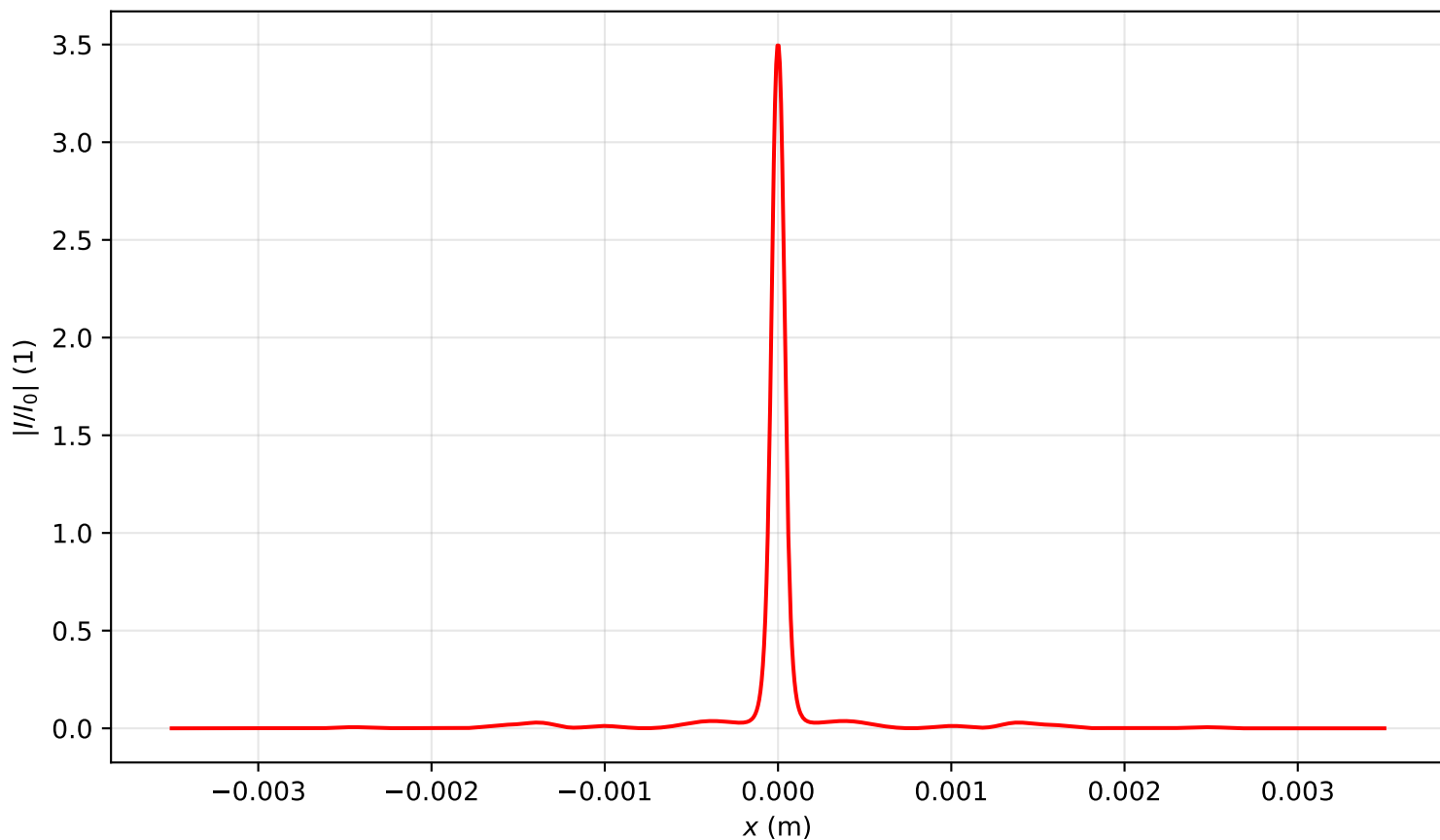
Intensity profile I(x, y = 0, z = 0.637)/I_0 , P_{in}=18.0P_{cr} , artificial time
