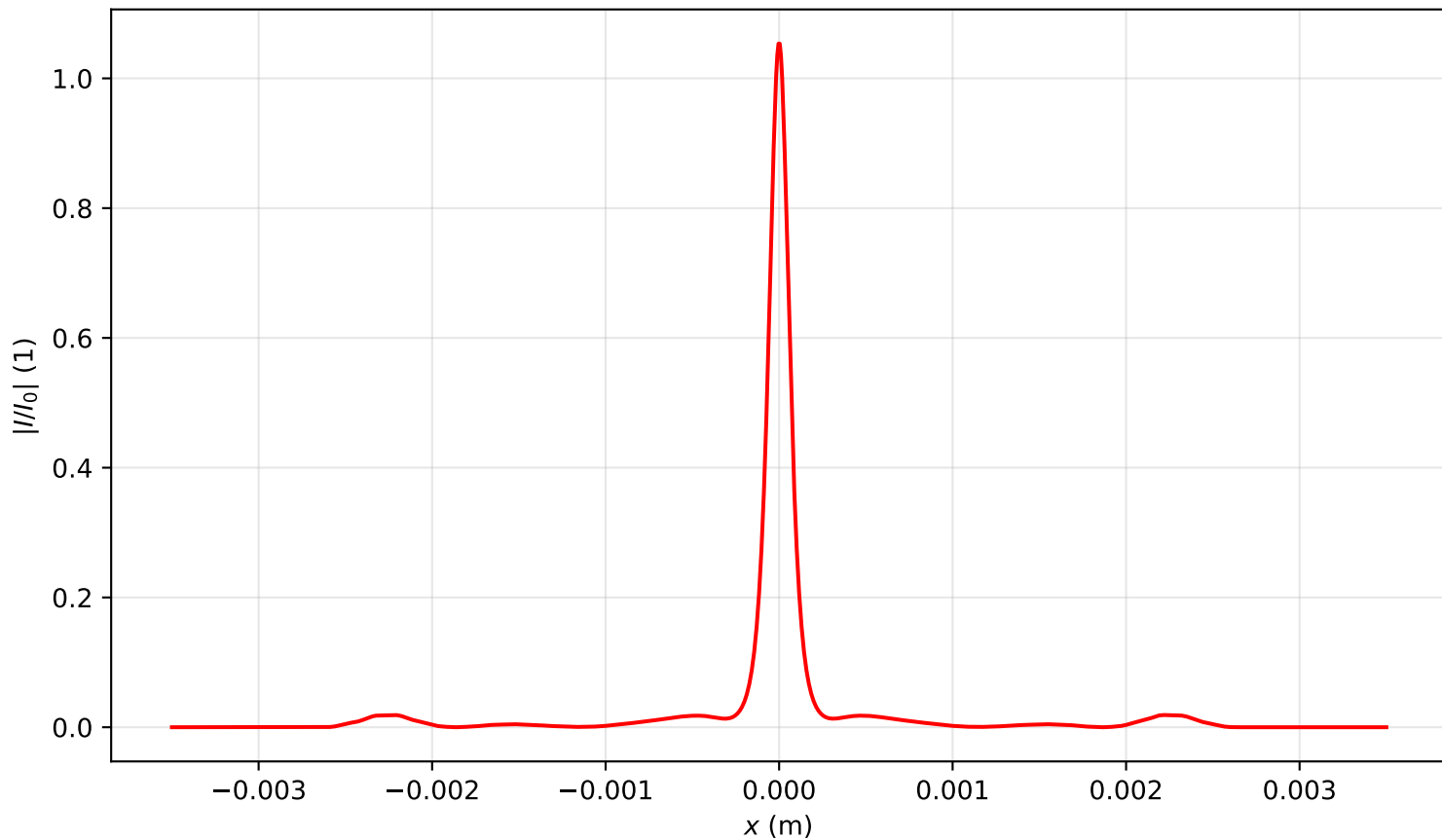
Intensity profile I(x, y = 0, z = 0.955)/I_0 , P_{in}=18.0P_{cr} , artificial time
