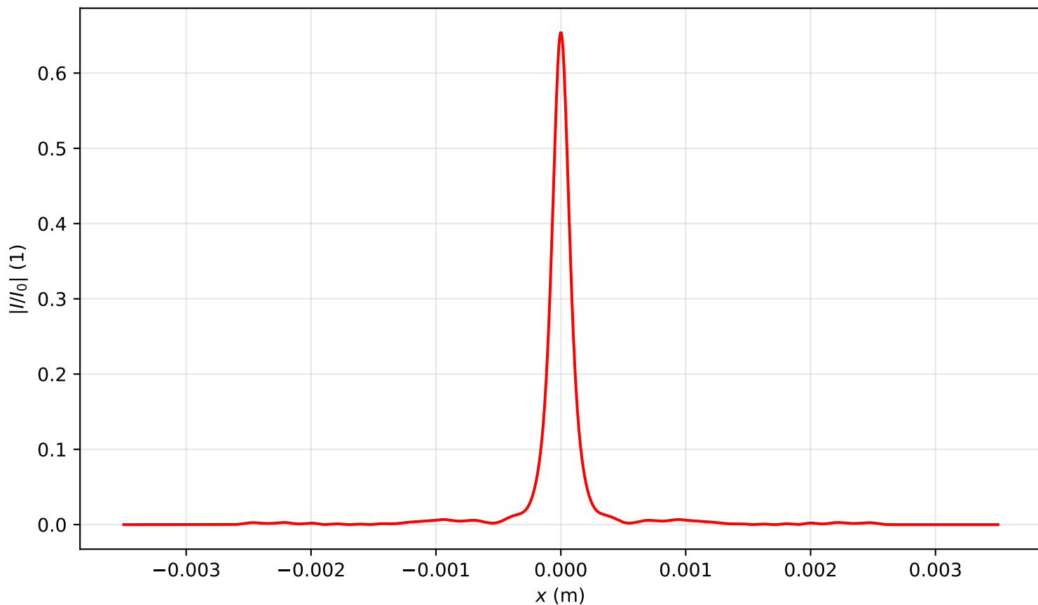
Intensity profile I(x, y = 0, z = 1.433)/I_0 , P_{in}=18.0P_{cr} , artificial time
