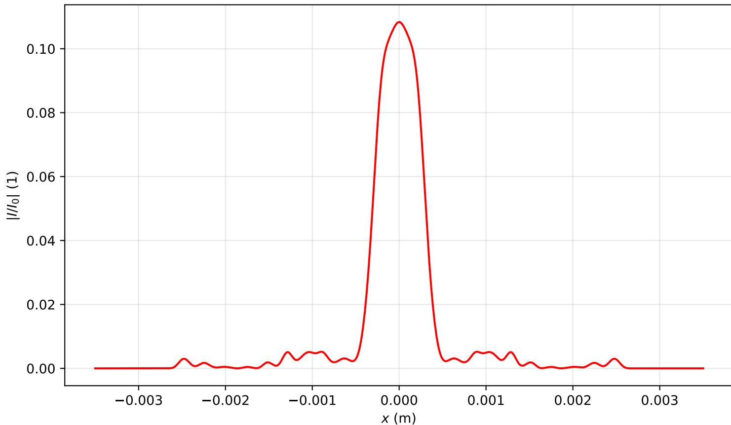
Intensity profile I(x, y = 0, z = 1.592)/I_0 , P_{in}=18.0\text{Pcr} , artificial time
