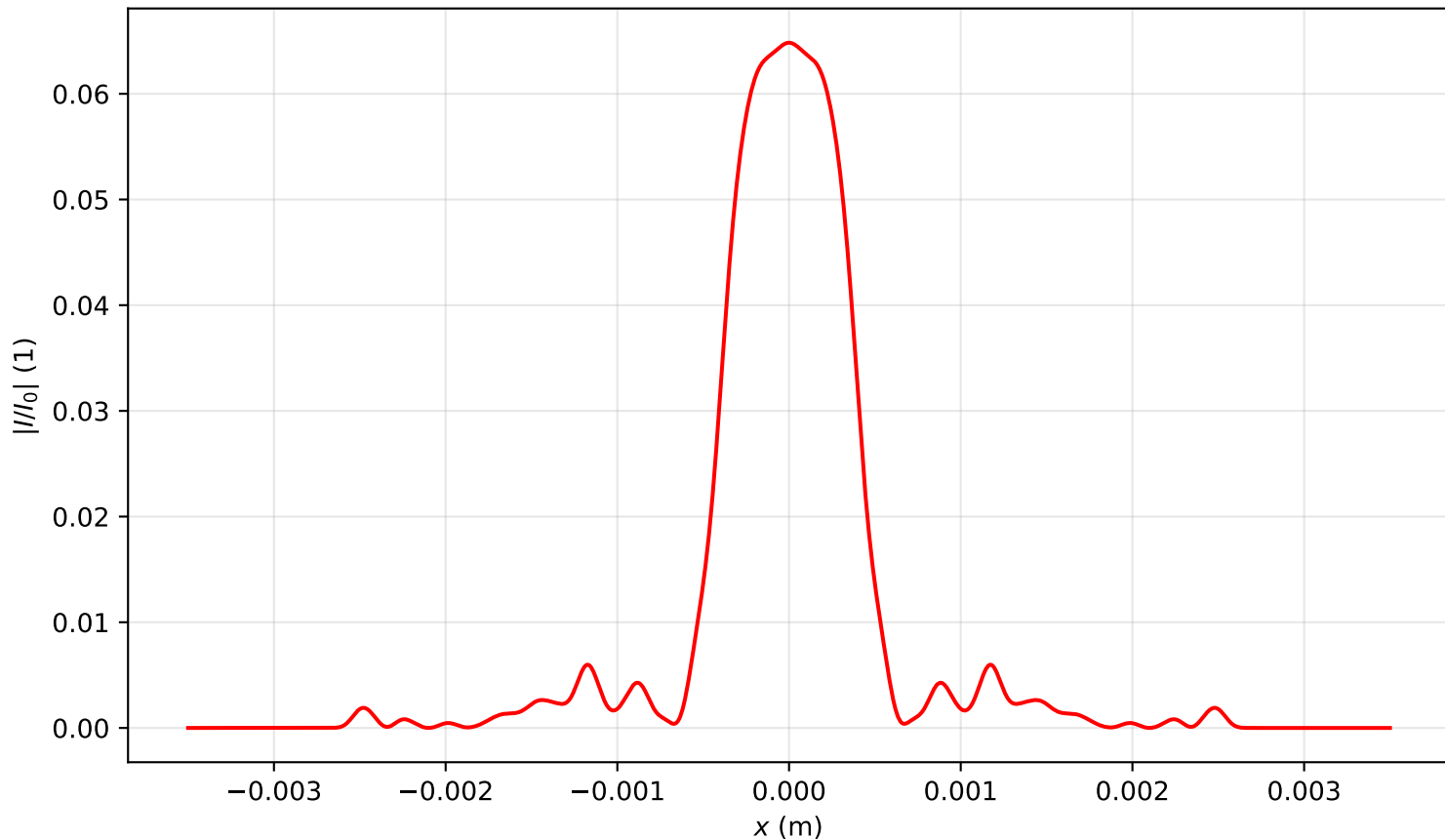
Intensity profile I(x, y = 0, z = 1.751)/I_0 , P_{in}=18.0P_{cr} , artificial time
