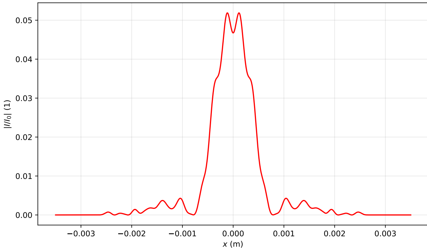
Intensity profile I(x, y = 0, z = 1.911)/I_0 , P_{in}=18.0\text{Pcr} , artificial time
