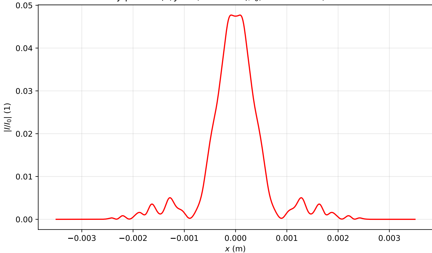
Intensity profile I(x, y = 0, z = 2.070)/I_0 , P_{in}=18.0\text{Pcr} , artificial time
