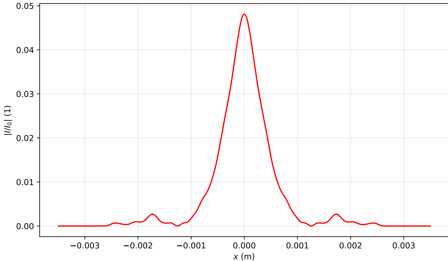
Intensity profile I(x, y = 0, z = 2.548)/I_0 , P_{in}=18.0\text{Pcr} , artificial time
