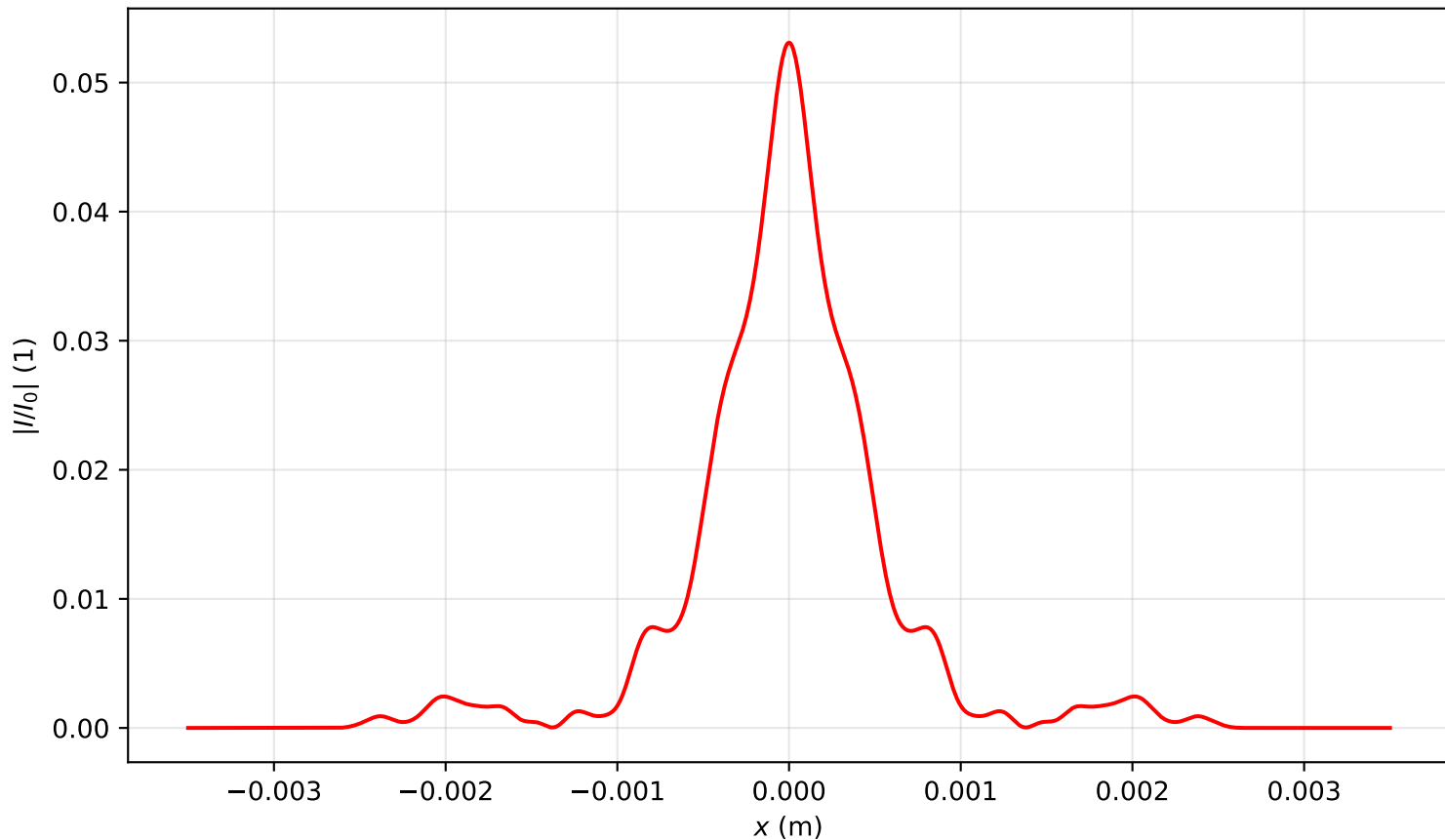
Intensity profile I(x, y = 0, z = 2.707)/I_0 , P_{in}=18.0\text{Pcr} , artificial time
